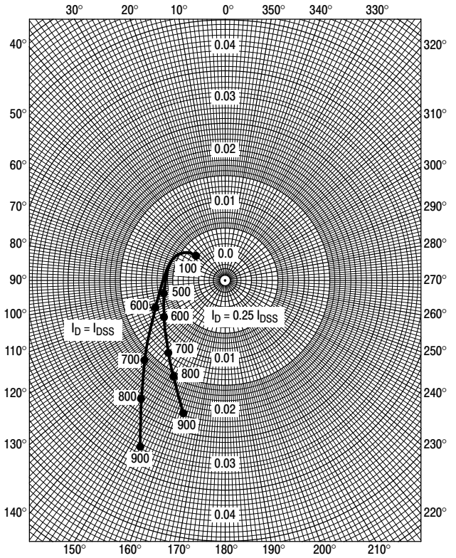
Figure 14. S_{12g}
