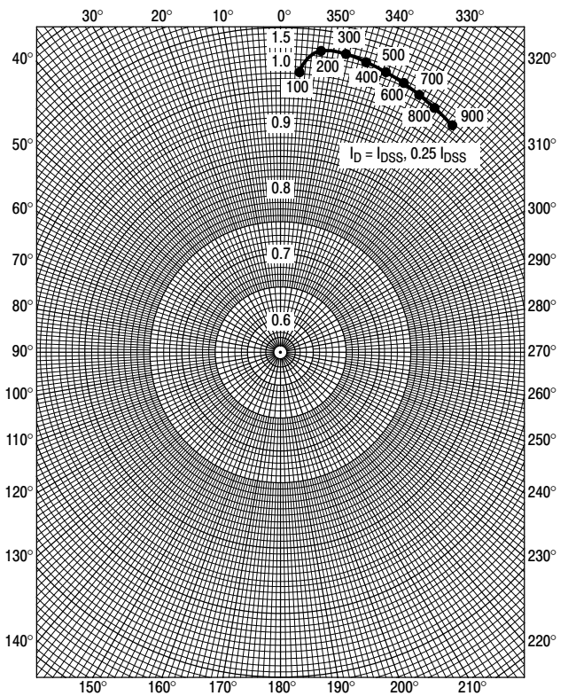
Figure 16. S_{22g}
