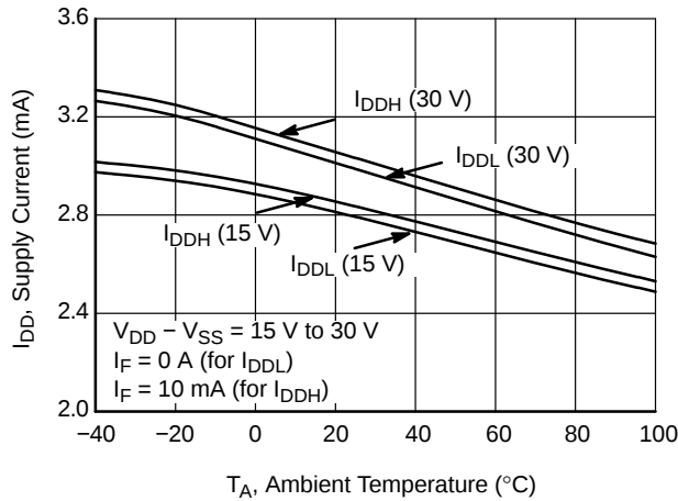
Figure 10. Supply Current vs. Ambient Temperature
