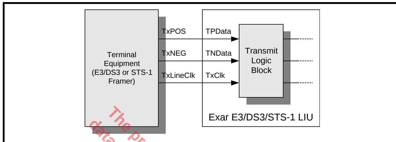
FIGURE 3. TYPICAL INTERFACE BETWEEN TERMINAL EQUIPMENT AND THE XRT75L00 (DUAL-RAIL DATA)
