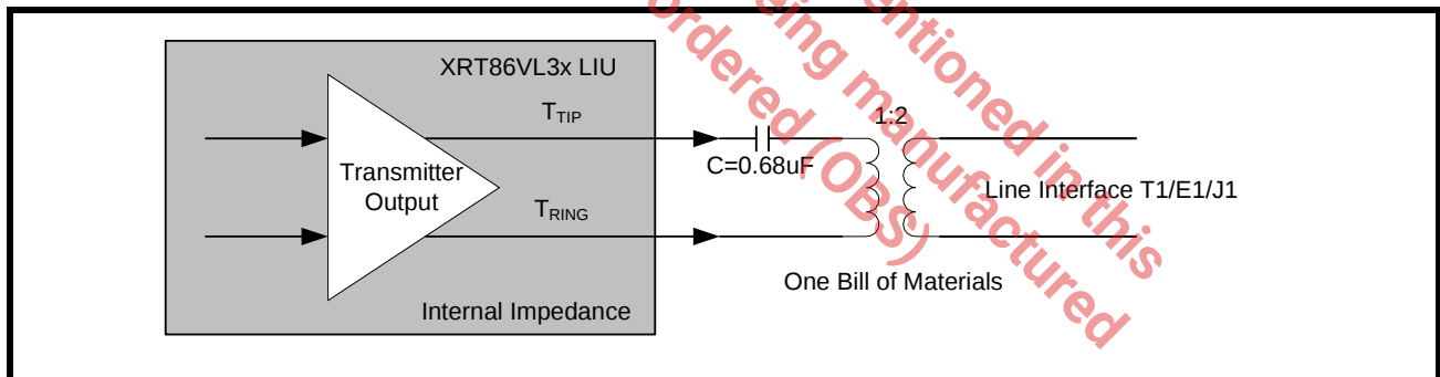
FIGURE 54. TYPICAL CONNECTION DIAGRAM USING INTERNAL TERMINATION
