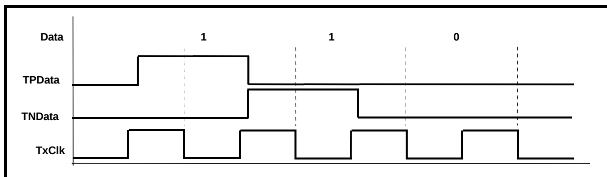
FIGURE 15. THE XRT73LC04A SAMPLES THE DATA ON THE TPDATA AND TNDAATA INPUT PINS
