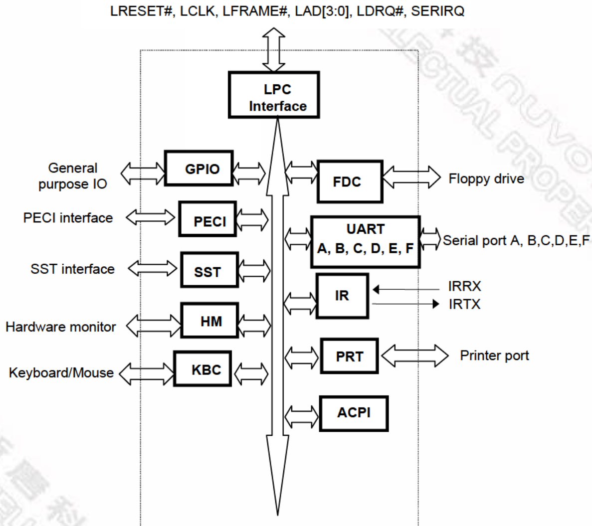
Figure 3-1 W83627UHG and NCT6627UD Block Diagram
