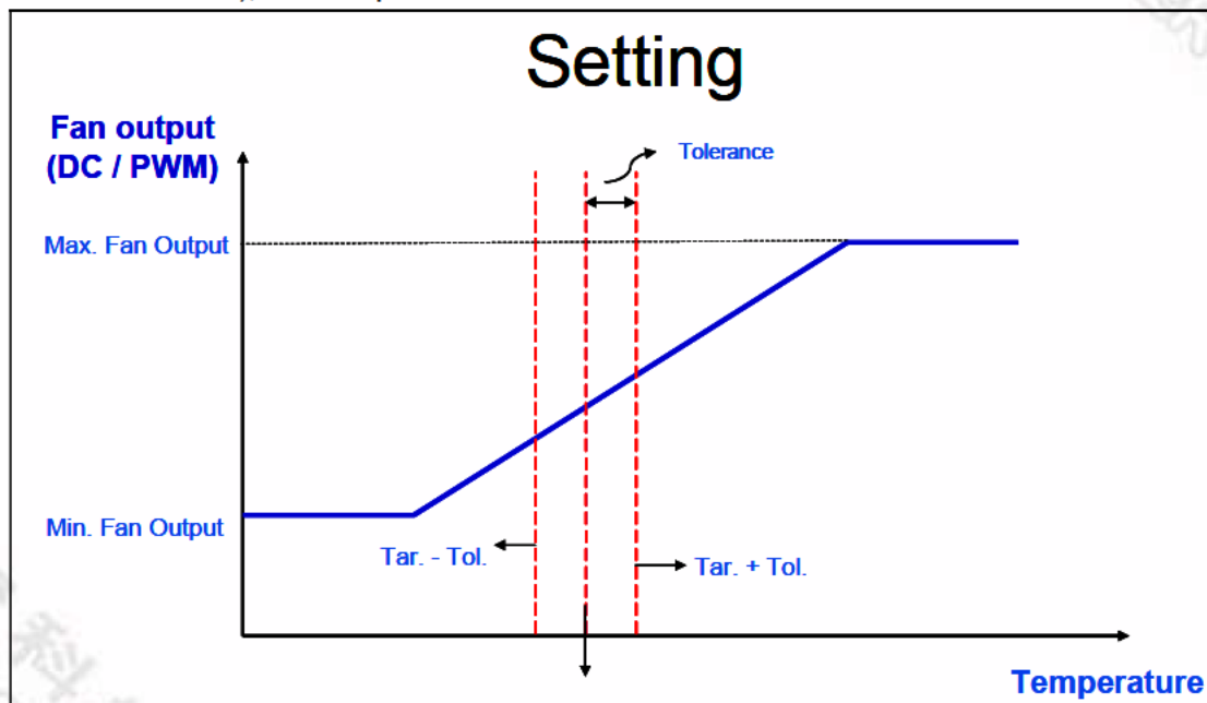
Figure 7-14 Setting of SMART FAN™ III
