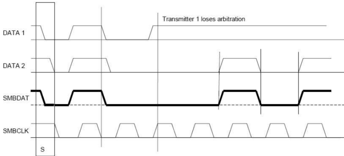
Figure 18-2 SMBus Arbitration
