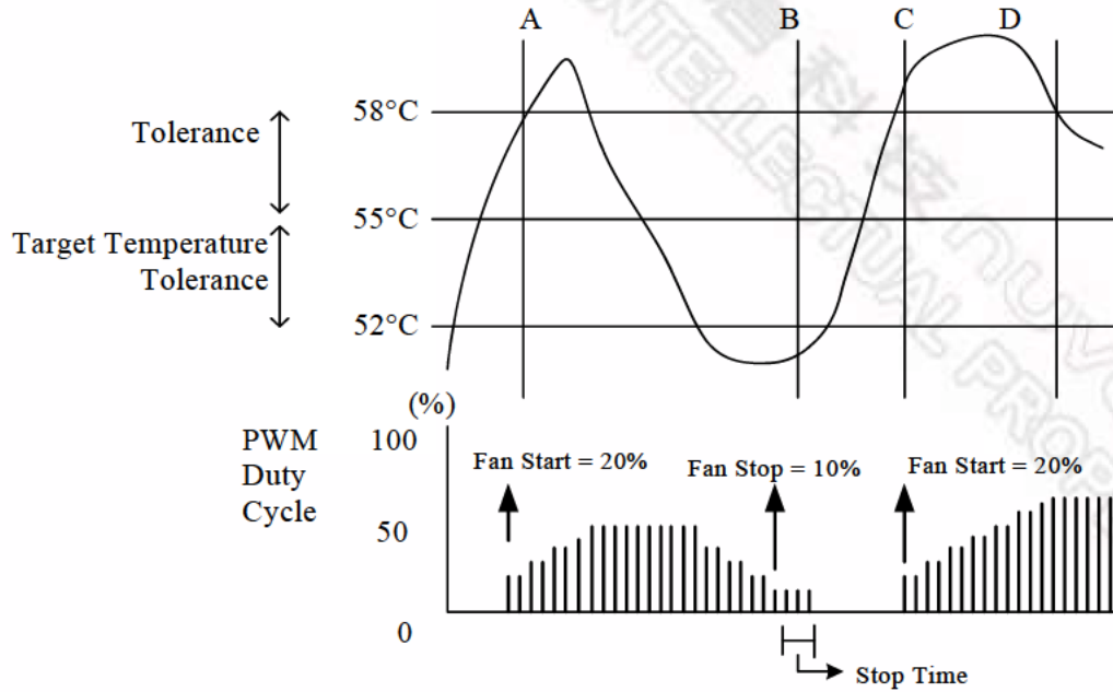
Figure 8-10 Mechanism of Thermal Cruise™ Mode (PWM Duty Cycle)
