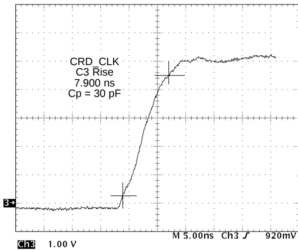
Figure 29. Card Clock Rise and Fall Time
