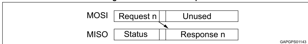
Figure 46. In-frame example
