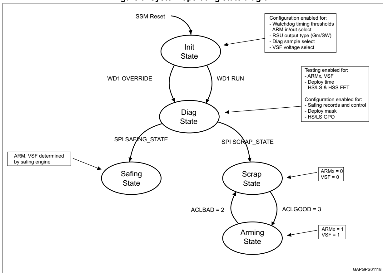
Figure 9. System operating state diagram
