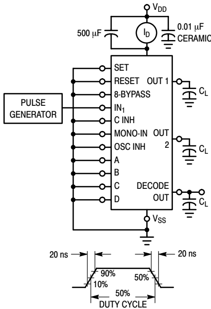
Figure 7. Power Dissipation Test Circuit and Waveform
