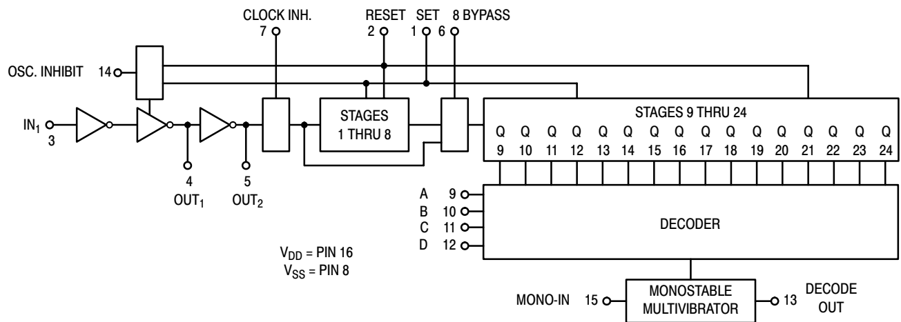
Figure 1. Block Diagram
