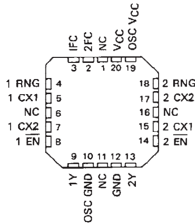
SN54S124 ... FK PACKAGE (TOP VIEW)
