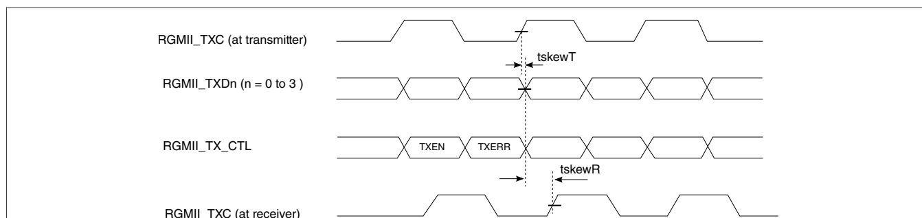
Figure 33. RGMII transmit signal timing diagram original
