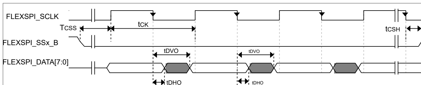
Figure 48. FlexSPI output timing in SDR mode
