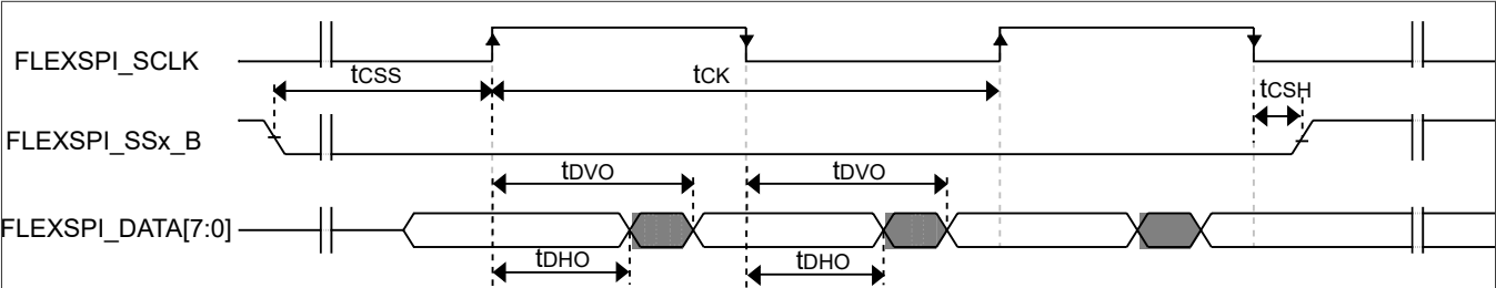
Figure 49. FlexSPI output timing in DDR mode
