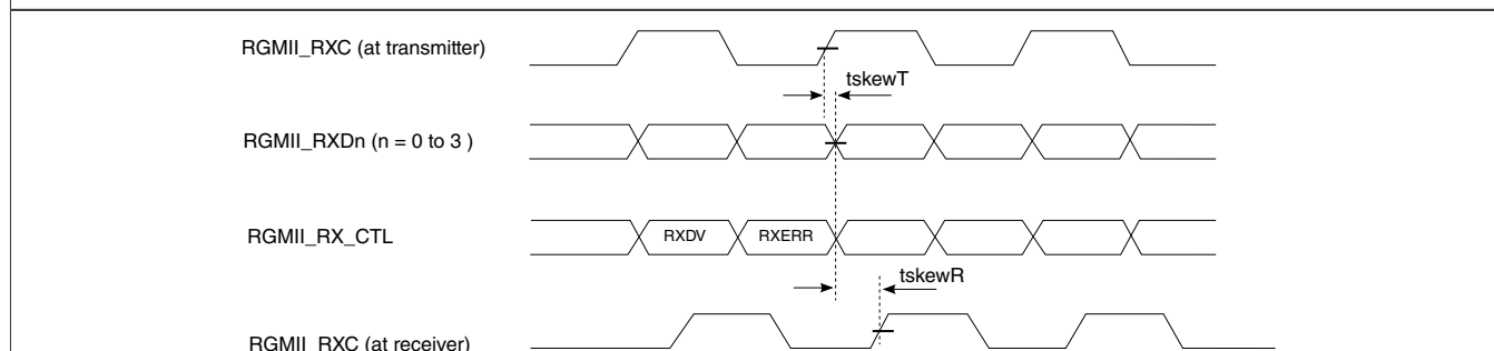
Figure 34. RGMII receive signal timing diagram original
