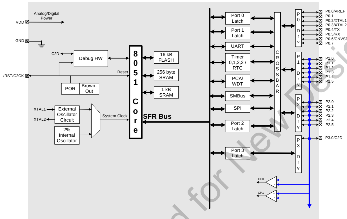
Figure 1.8. C8051F317 Block Diagram
