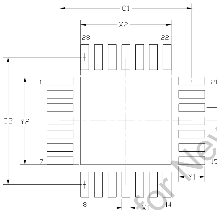
Figure 4.6. Typical QFN-28 Landing Diagram
