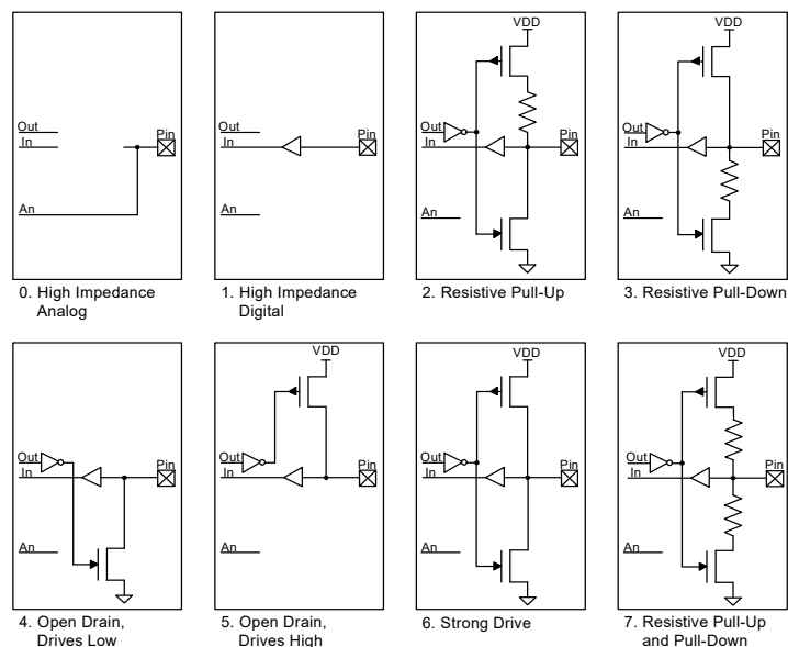
Figure 6-12. Drive Mode
