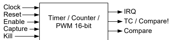
Figure 7-15. Timer/Counter/PWM
