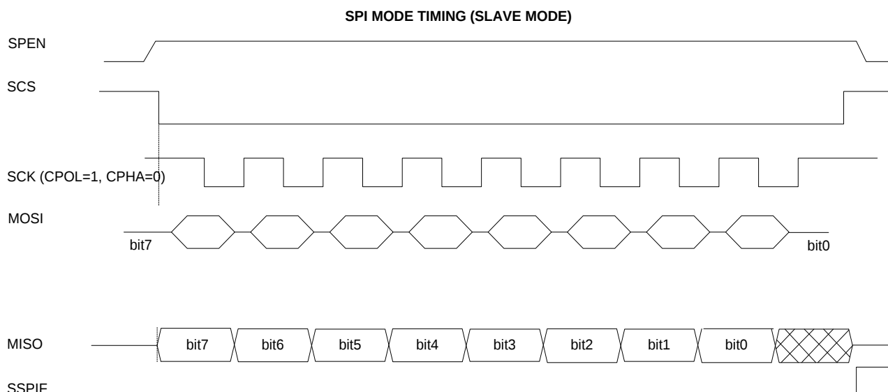
Figure 10-7 SPI Slave Timing with CPOL=1. CPHA=0
