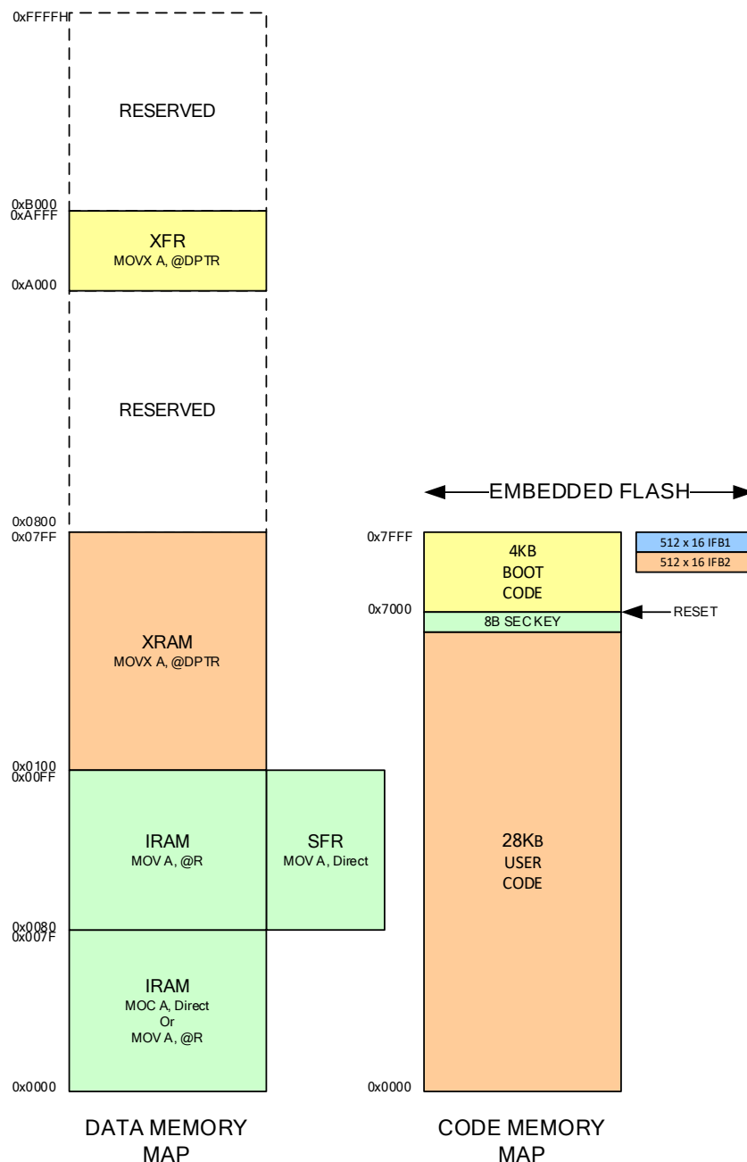
Figure 2-1 Memory Map
