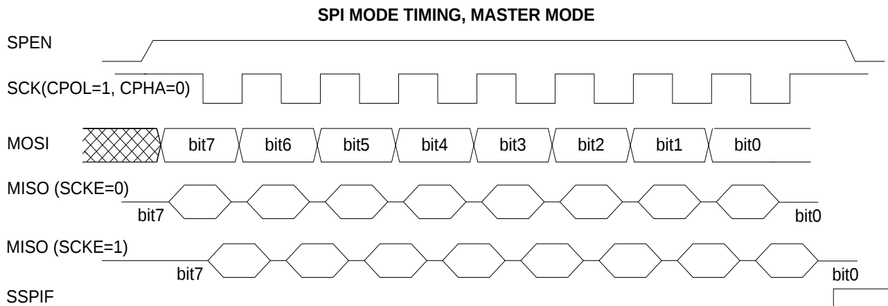
Figure 10-3 SPI Master Timing with CPOL=1, CPHA=0
