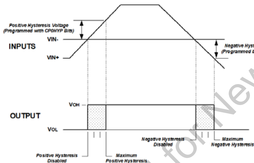
Figure 7.2. Comparator Hysteresis Plot
