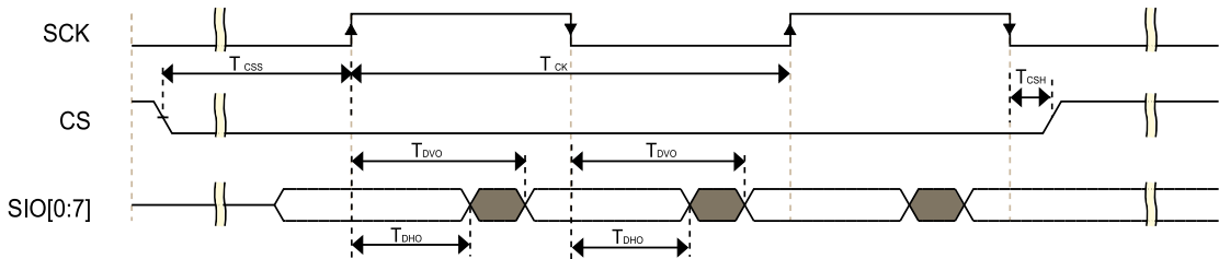
Figure 21. FlexSPI output timing in DDR mode
