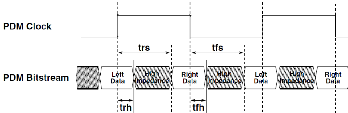
Figure 51. Input/Output Timing Requirements
