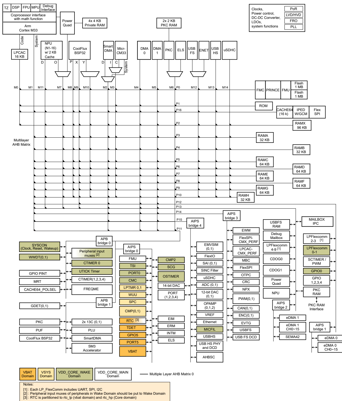
Figure 2. MCX N9xx/N5xx/N24x Architecture
