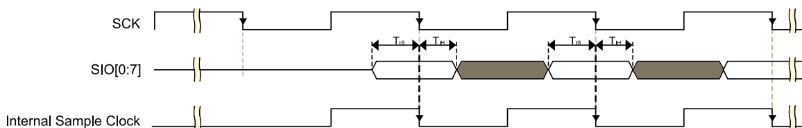
Figure 14. FlexSPI input timing in SDR mode where FlexSPI \overline{n} _MCR0[RXCLKSRC] = 0x0 or 0x1 or 0x2
