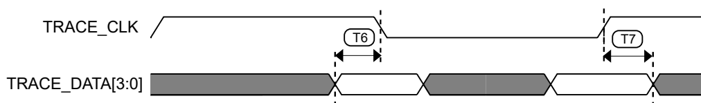
Figure 7. Trace data specifications
