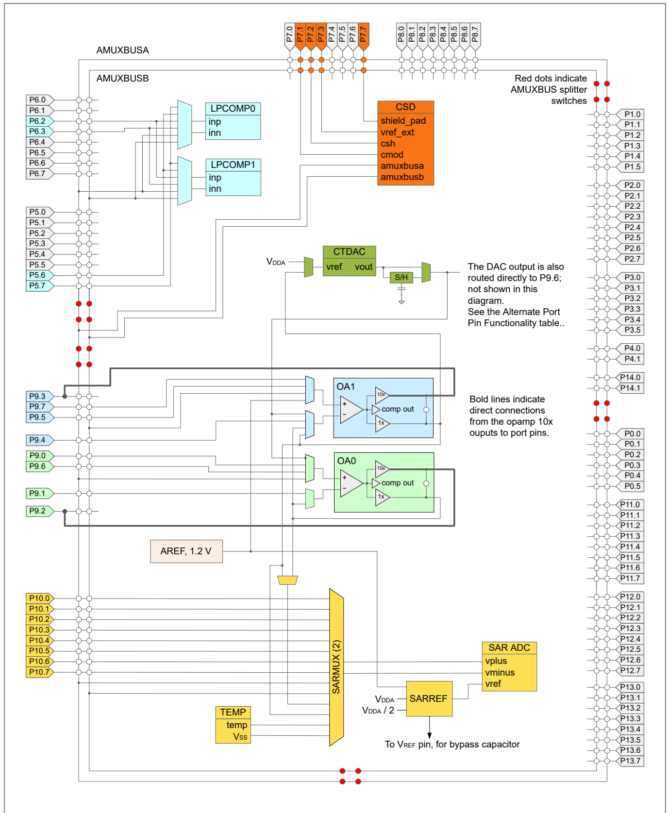
Figure 7 Analog subsystem
