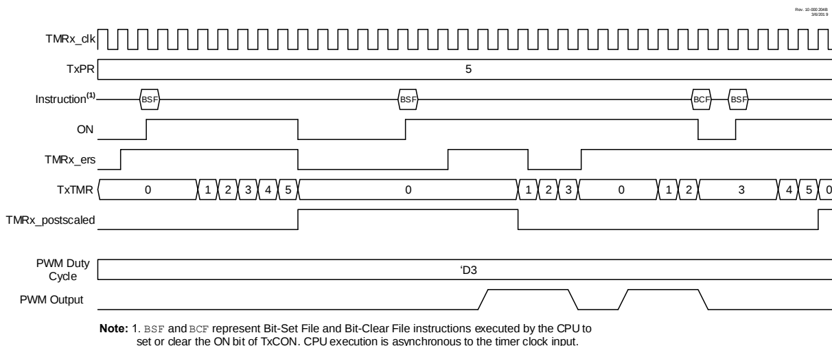
Figure 25-12. Level Triggered Hardware Limit One Shot Mode Timing Diagram (MODE = 'b10110)
