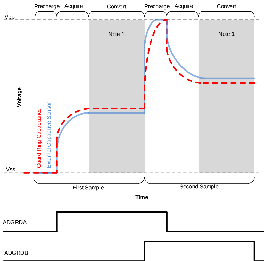
Figure 35-15. Differential CVD with Guard Ring Output Waveform
