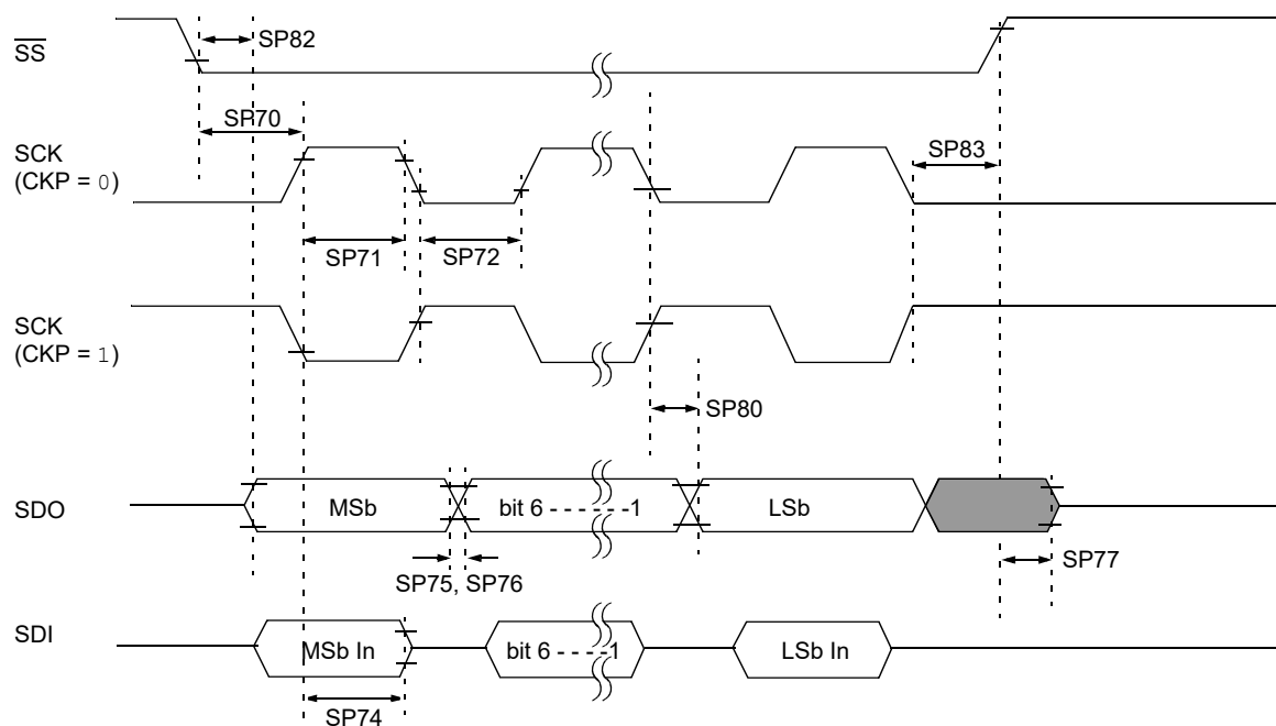
Figure 48-18. SPI Client Mode Timing (CKE = 1)
