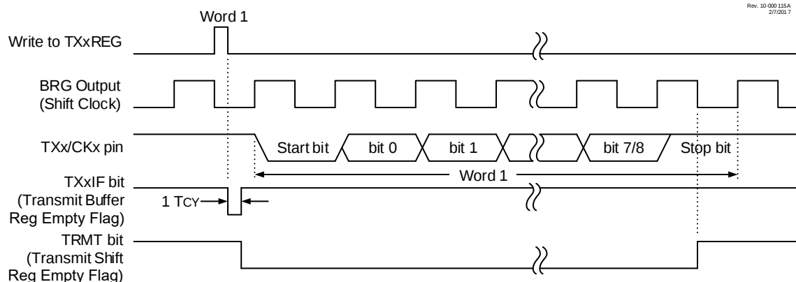
Figure 33-10. Synchronous Transmission
