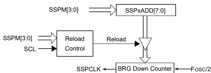
Figure 32-41. Baud Rate Generator Block Diagram
