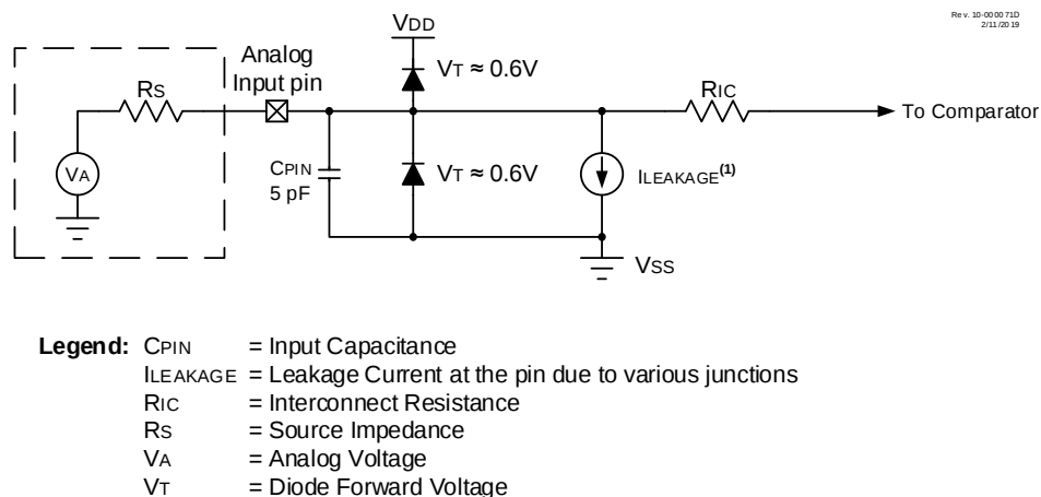
Figure 38-3. Analog Input Model
