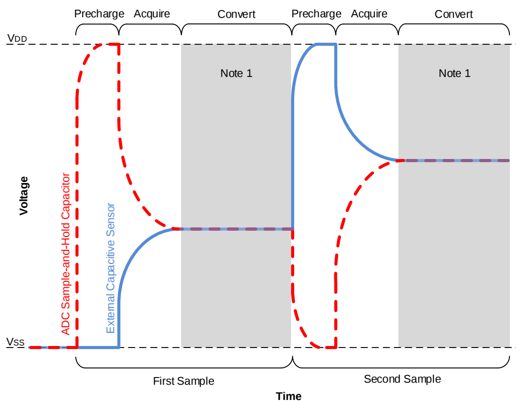
Figure 35-13. Differential CVD Measurement Waveform
