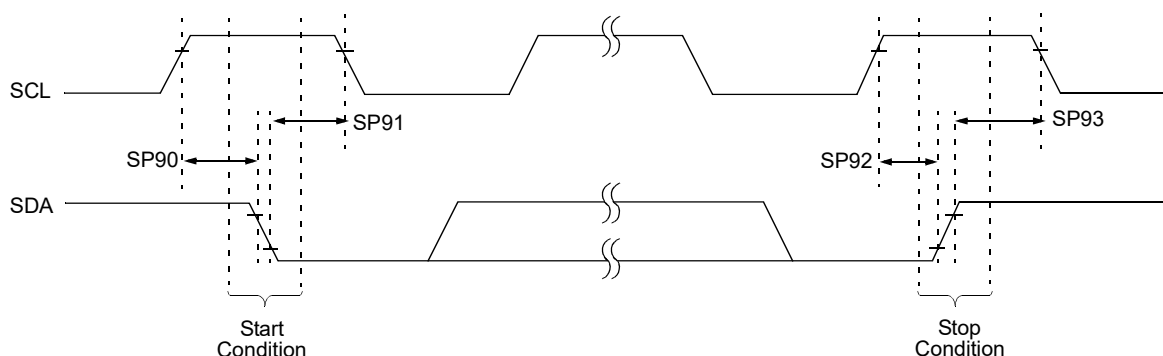
Figure 48-19. I 2 C Bus Start/Stop Bits Timing
