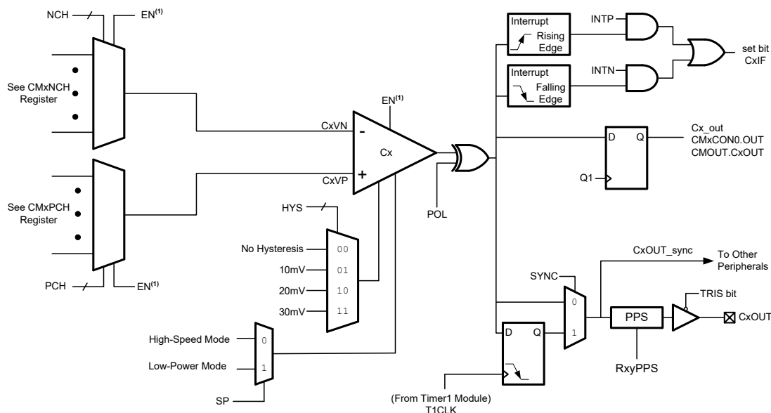
Figure 38-2. Comparator Module Simplified Block Diagram
