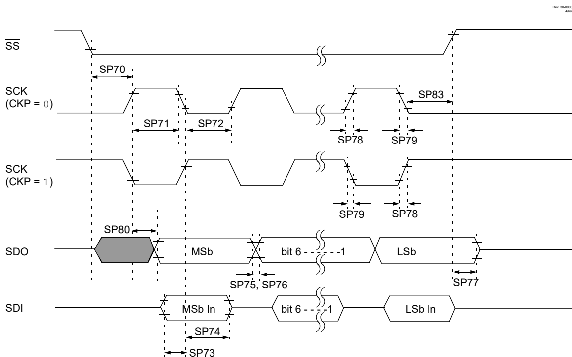
Figure 48-17. SPI Client Mode Timing (CKE = 0)
