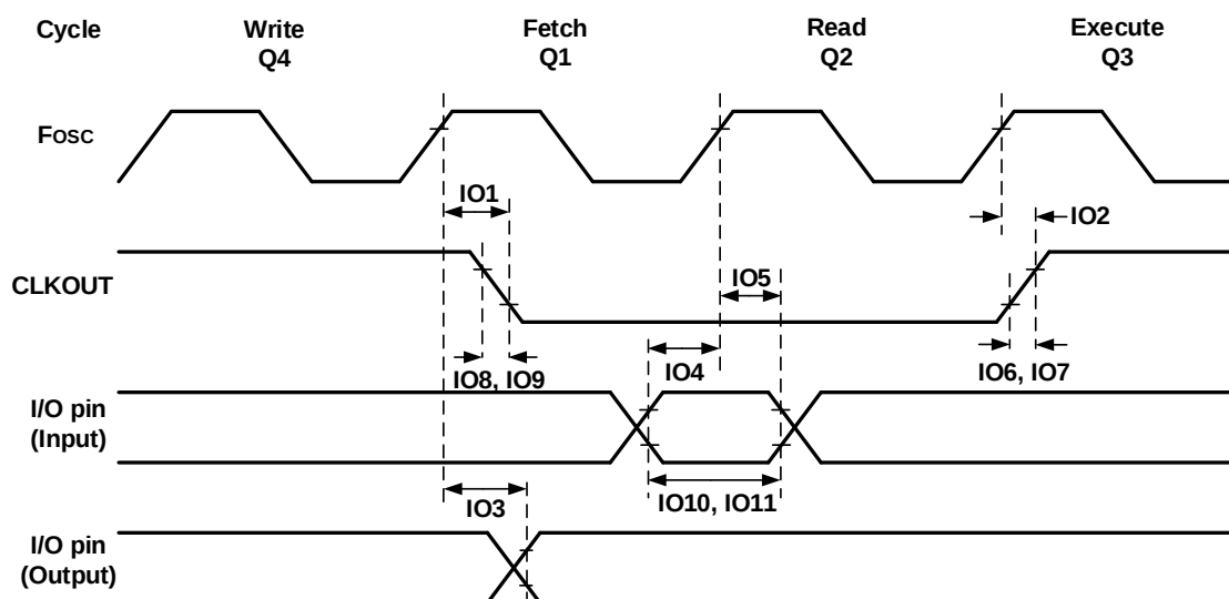
Figure 48-6. CLKOUT and I/O Timing
