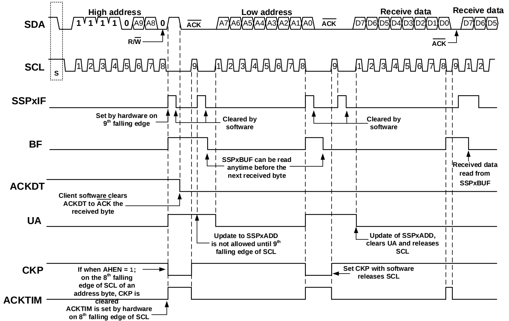
Figure 32-20. I 2 C Client, 10-Bit Address, Reception (SEN = 0, AHEN = 1, DHEN = 0)
