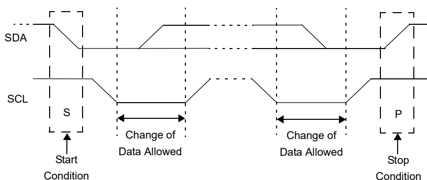
Figure 32-12. I 2 C Start and Stop Conditions
