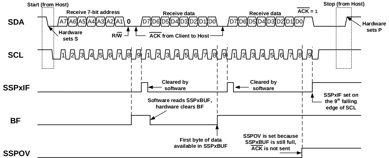
Figure 32-15. I 2 C Client, 7-Bit Address, Reception (SEN = 0, AHEN = 0, DHEN = 0)
