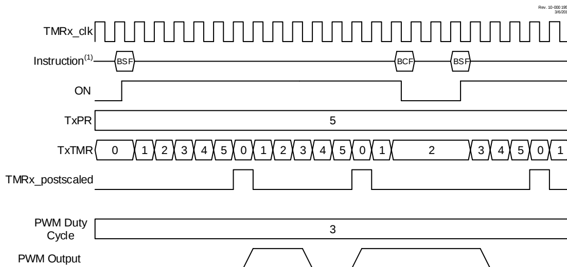
Figure 25-3. Software Gate Mode Timing Diagram ( MODE = 'b000000 )
