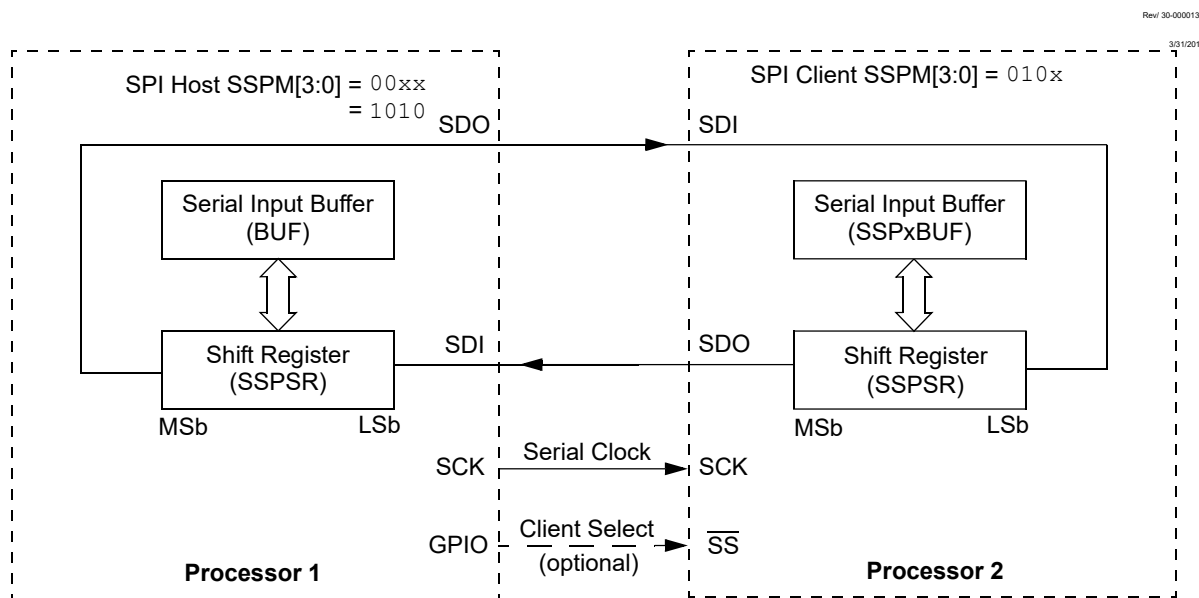
Figure 32-3. SPI Host/Client Connection
