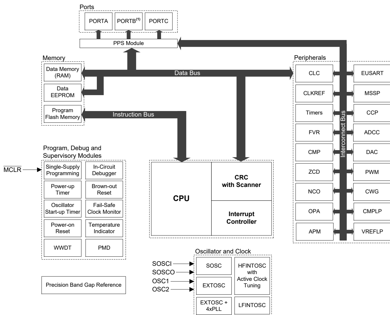
Figure 1. PIC16F17526/46 Block Diagram
