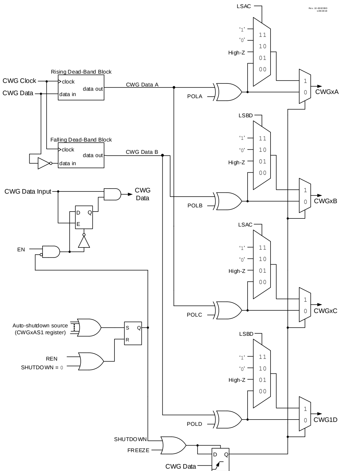
Figure 30-2. Simplified CWG Block Diagram (Half Bridge Mode, MODE = 'b100)
