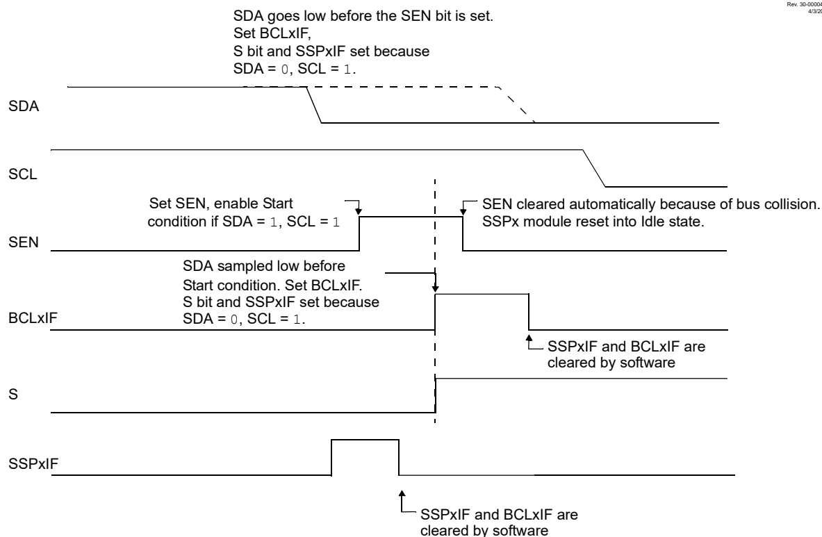
Figure 32-34. Bus Collision During Start Condition (SDA Only)
