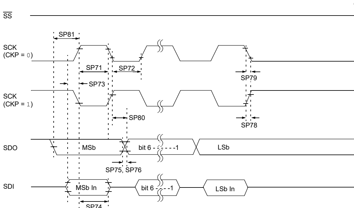
Figure 48-16. SPI Host Mode Timing (CKE = 1, SMP = 1)
