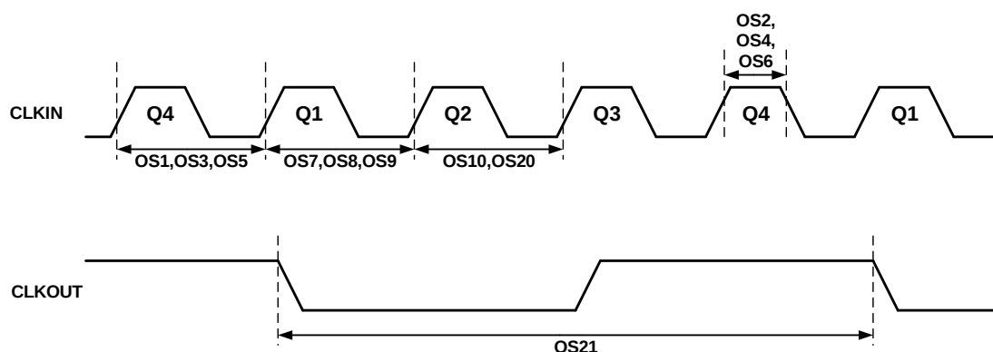
Figure 48-4. Clock Timing
