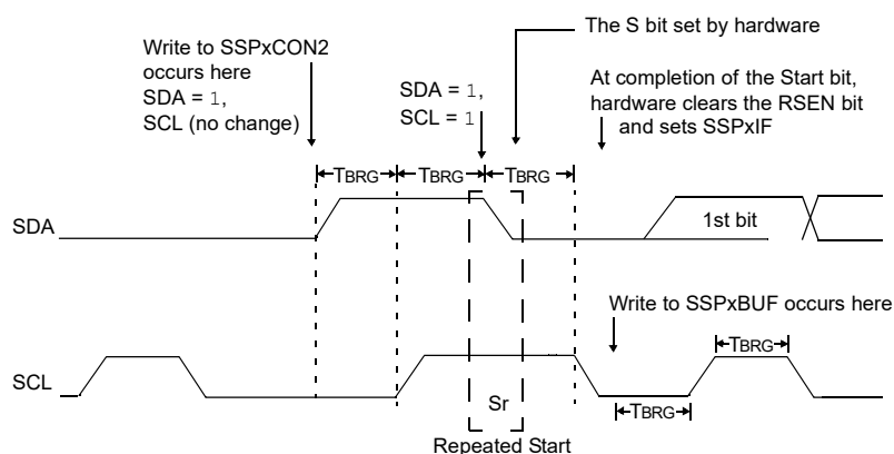
Figure 32-26. Repeated Start Condition Waveform
