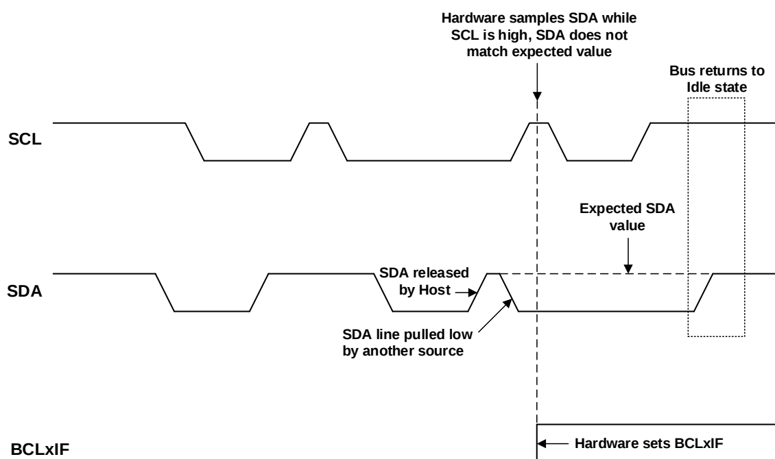
Figure 32-33. Bus Collision Timing for Transmit and Acknowledge
