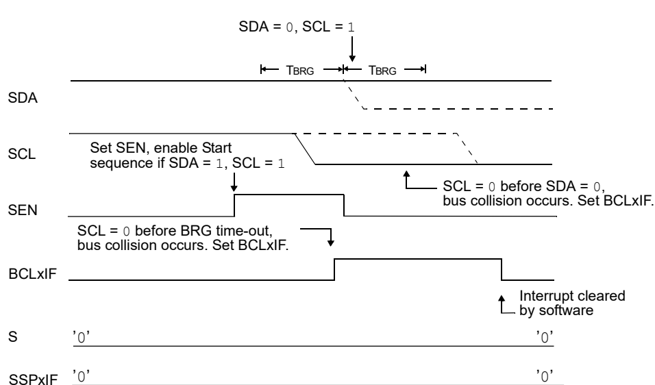
Figure 32-35. Bus Collision During Start Condition (SCL = 0)
