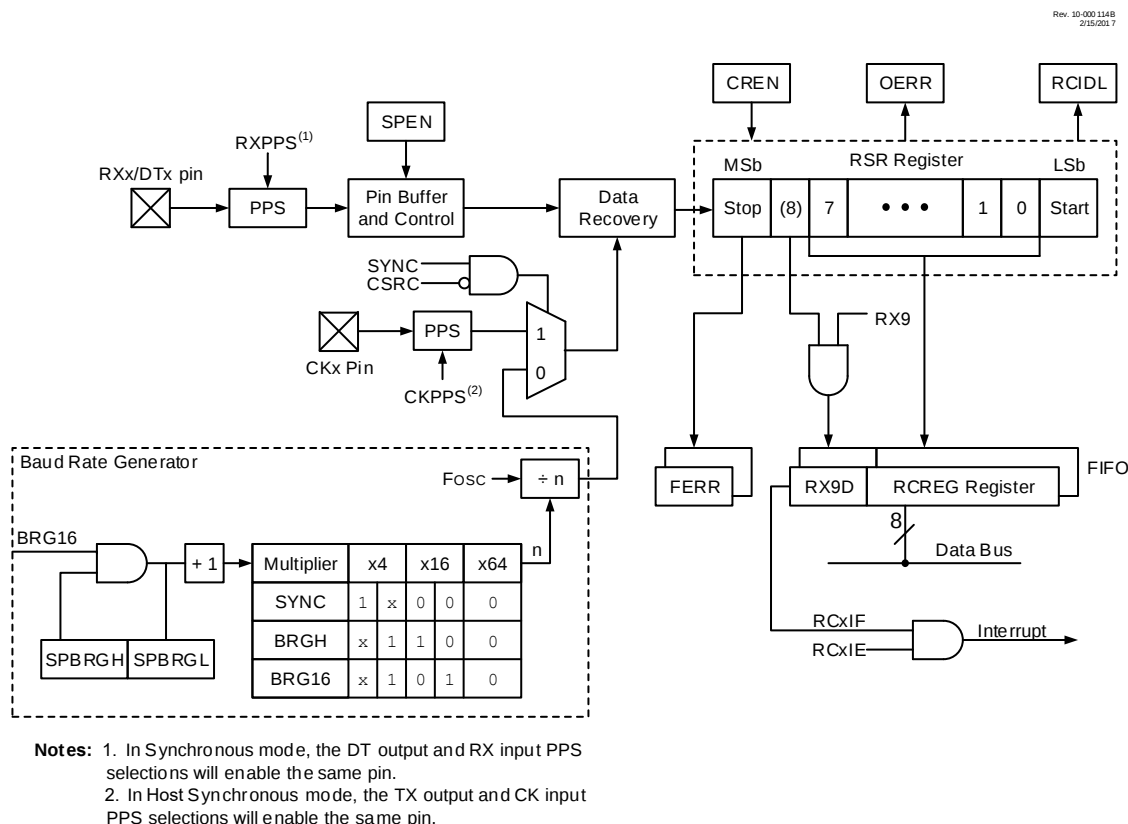
Figure 33-2. EUSART Receive Block Diagram
