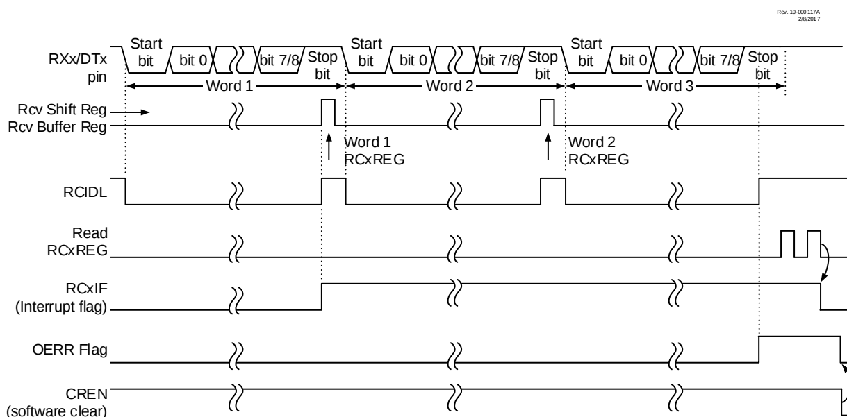
Figure 33-5. Asynchronous Reception
