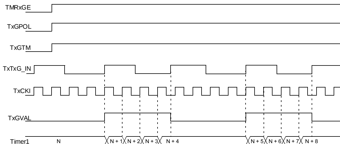
Figure 24-5. Timer1 Gate Toggle Mode
