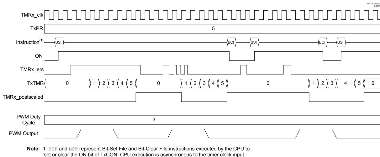
Figure 25-11. Rising Edge Triggered Monostable Mode Timing Diagram (MODE = 'b10001)
