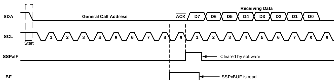
Figure 32-14. Client Mode General Call Address Sequence
