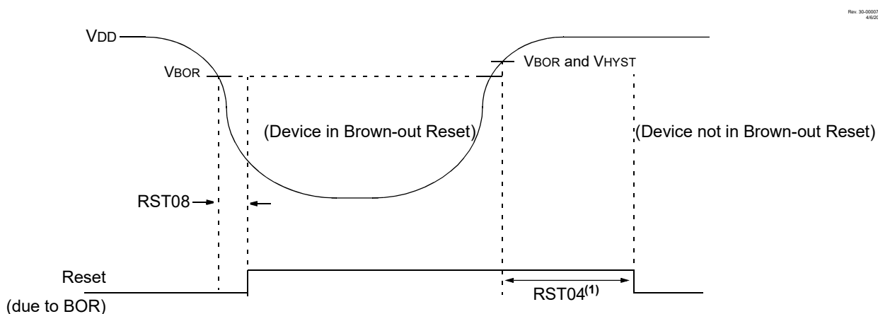
Figure 48-8. Brown-out Reset Timing and Characteristics
