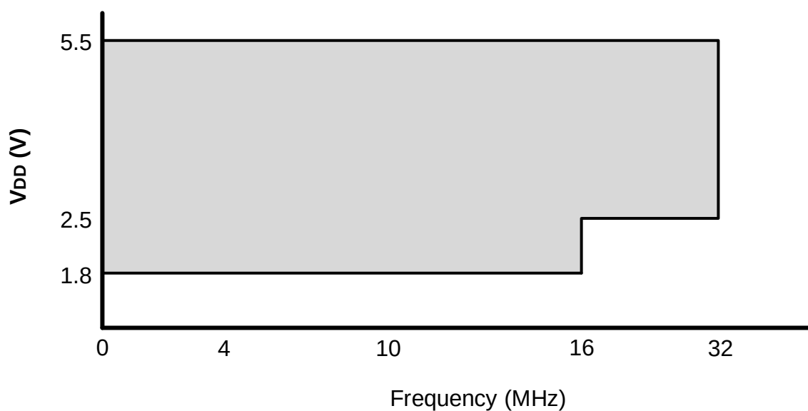
Figure 48-1. Voltage Frequency Graph, -40^{\circ}\text{C} \leq T_A \leq +125^{\circ}\text{C}
