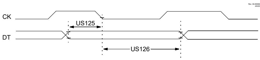
Figure 48-14. EUSART Synchronous Receive (Host/Client) Timing
