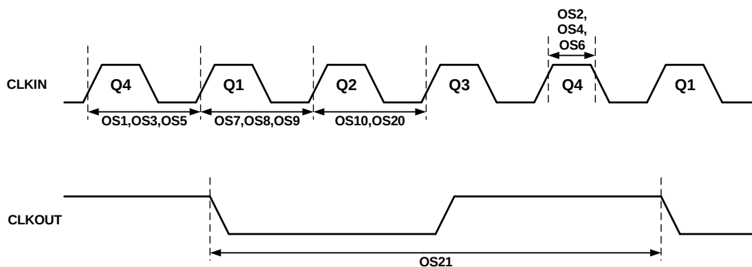
Figure 48-4. Clock Timing
