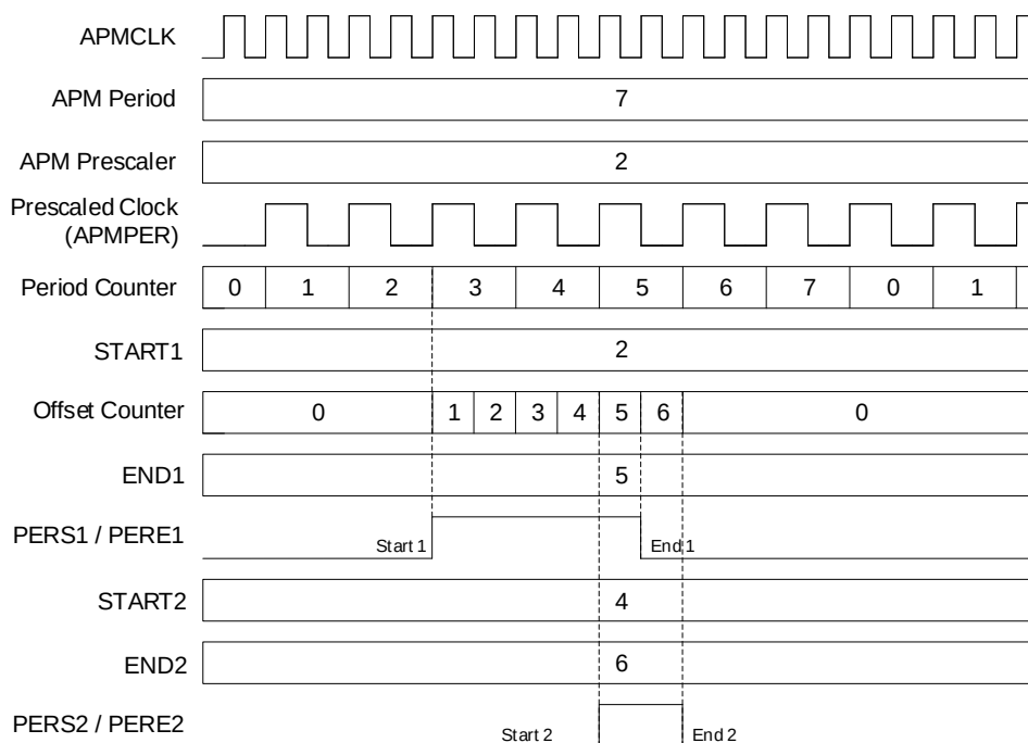
Figure 34-1. Analog Peripheral Manager Timing Diagram (APMPRE = 1 and APMPER = 7)
