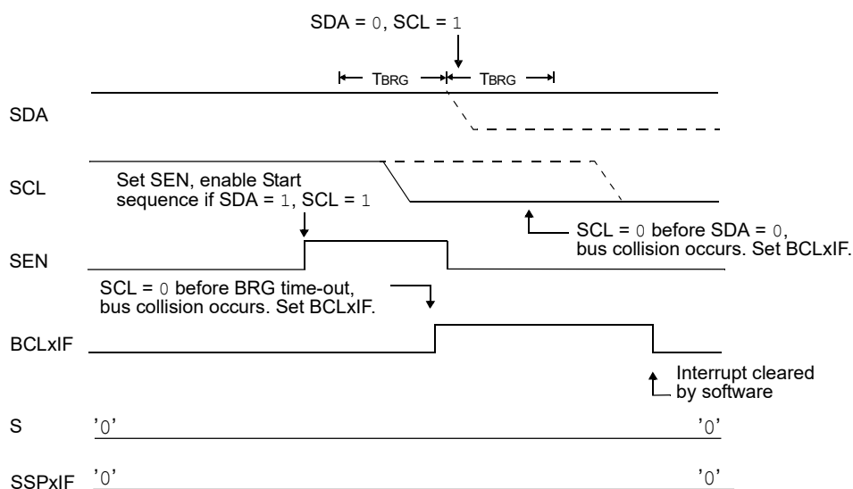
Figure 32-35. Bus Collision During Start Condition (SCL = 0)
