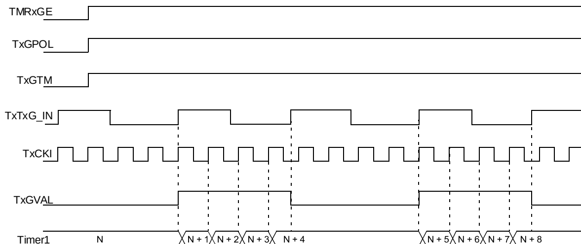
Figure 24-5. Timer1 Gate Toggle Mode
