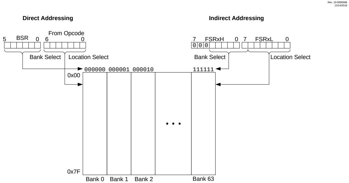
Figure 9-21. Traditional/Banked Data Memory Map
