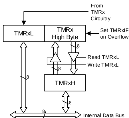
Figure 24-3. Timer1 16-Bit Read/Write Mode Block Diagram
