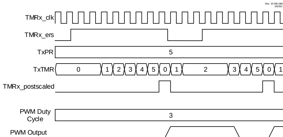
Figure 25-4. Hardware Gate Mode Timing Diagram ( MODE = \text{'b00001} )
