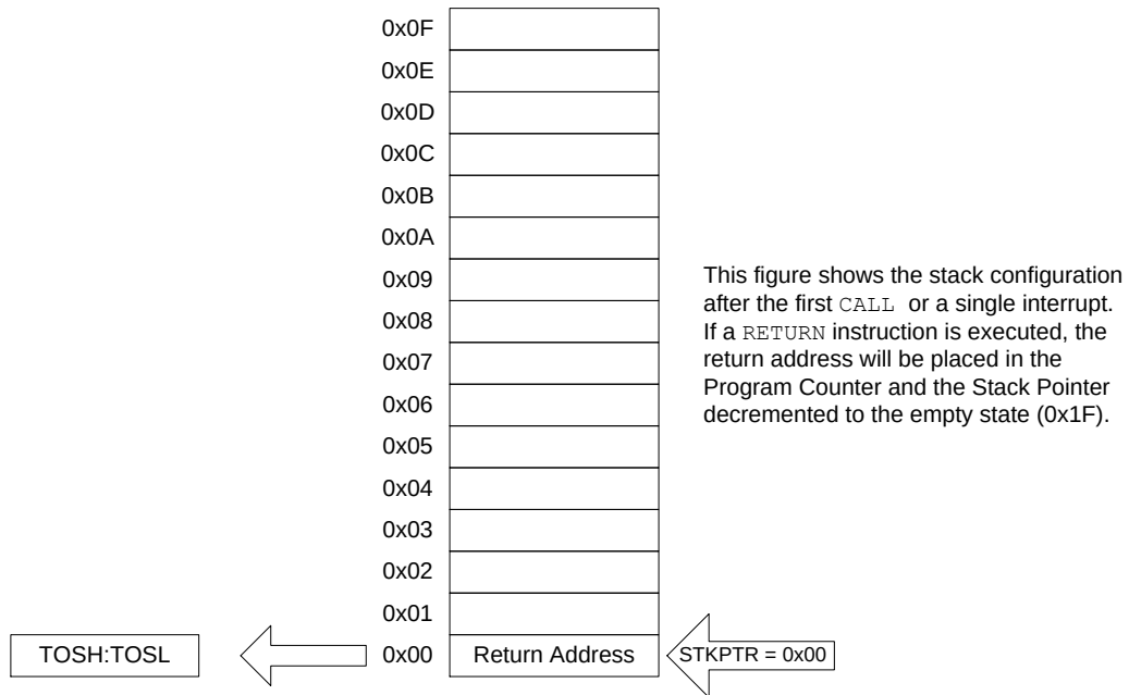
Figure 9-18. Accessing the Stack Example 3
