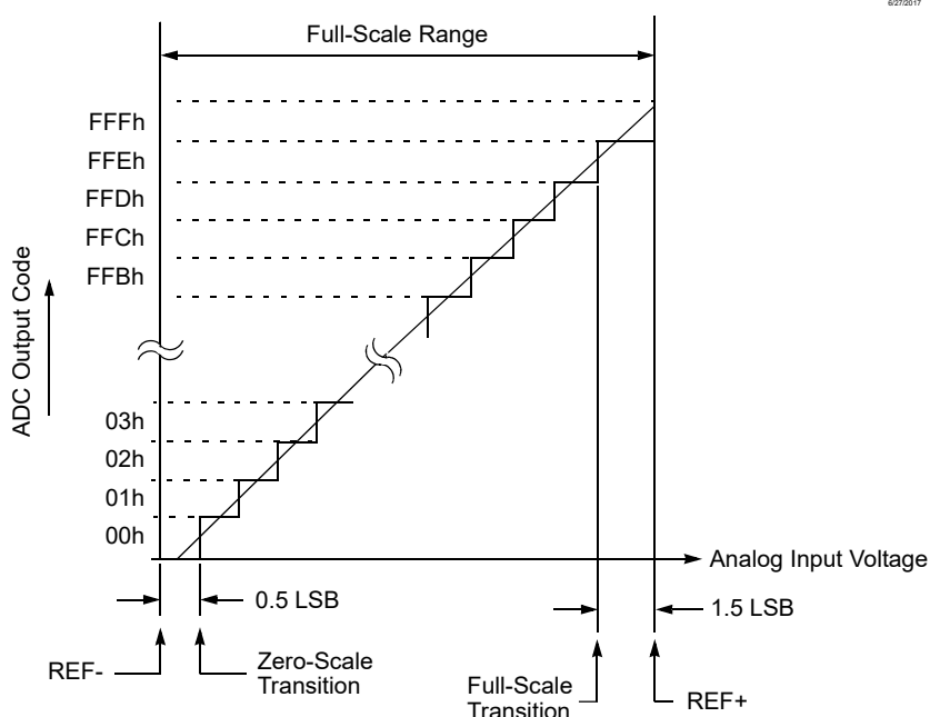
Figure 35-10. ADC Transfer Function
