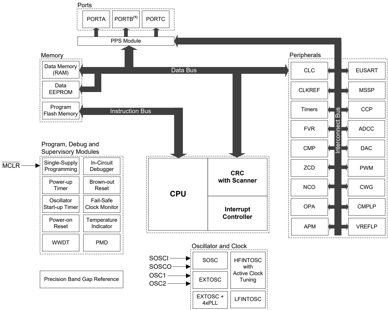
Figure 1. PIC16F17526/46 Block Diagram
