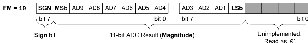
Figure 35-7. 12-Bit ADC Conversion Result Alignment/Format: IC = 1, FM = 10
