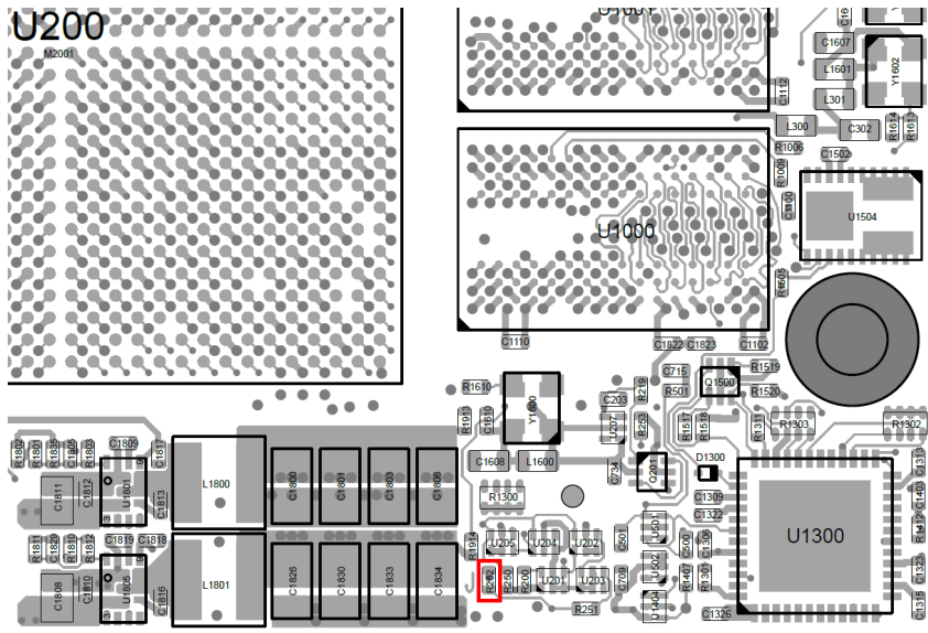
Figure 14: JTAG Boot Mode Resistor - Assembly Drawing Top View (lower right part)
