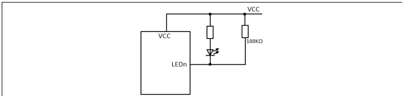
Figure 9. High Value Resistor in Parallel with the LED
