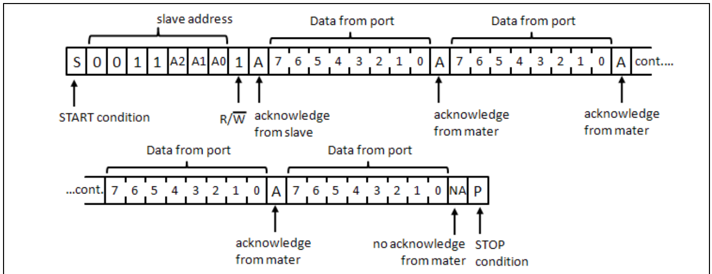
Figure 7. Read Input Port Register
