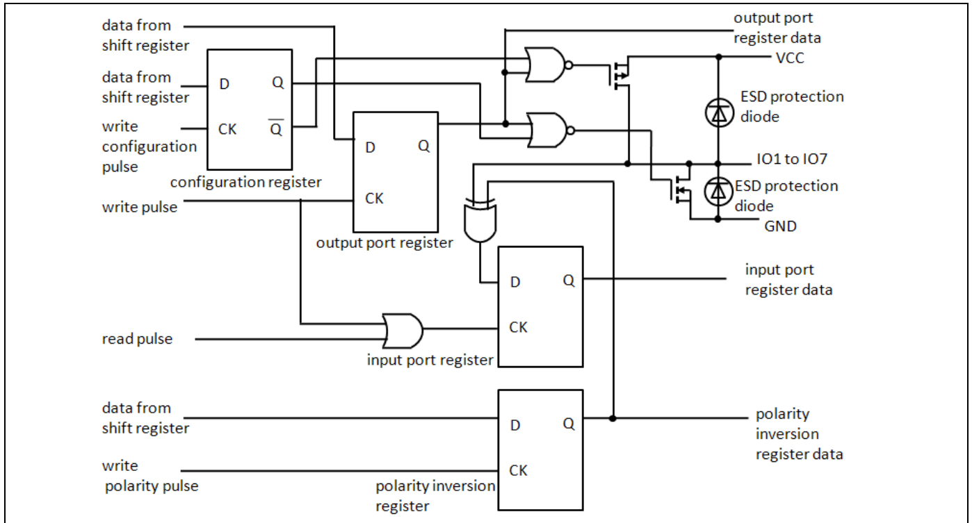
Figure 3. Simplified Schematic of IO1 to IO7
