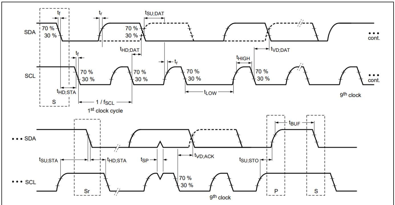
Figure 1. Diagram for Fast Speed Mode Devices on the I2C Bus.
