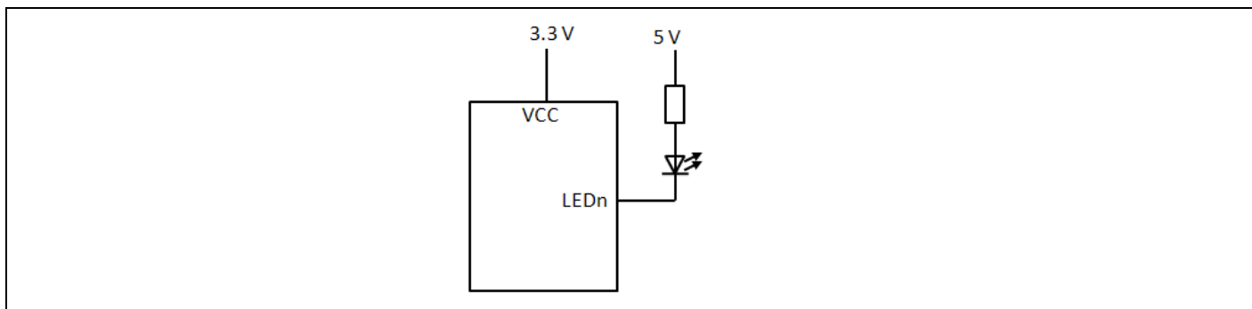
Figure 10. Device Supplied by a Lower Voltage
