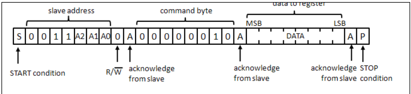
Figure 5. Write to I/O Configuration or Polarity Inversion Registers
