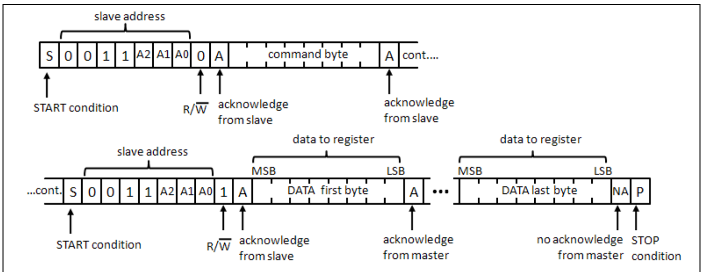
Figure 6. Read from Register
