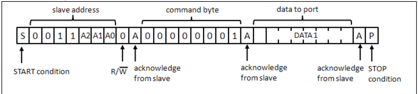
Figure 4. Write to Output Registers
