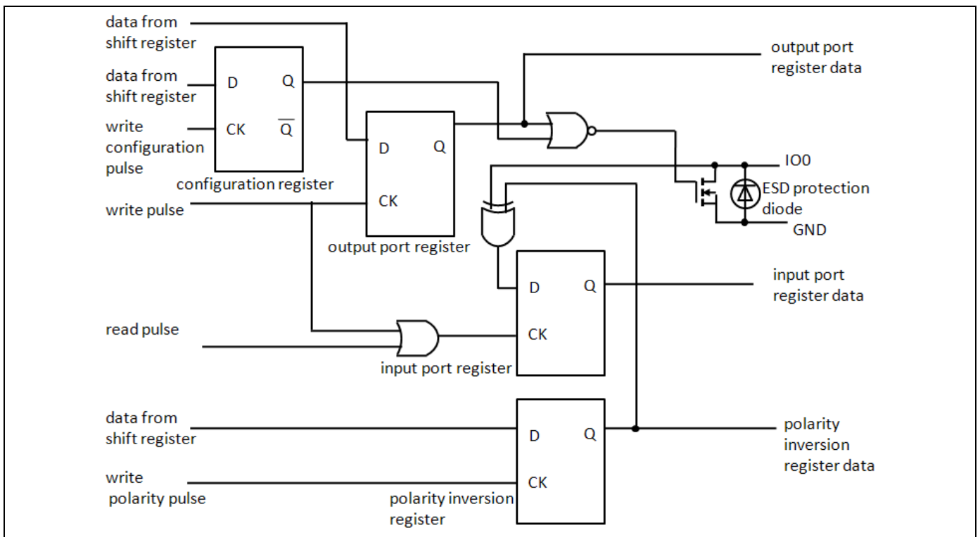
Figure 2. Simplified Schematic of IO0
