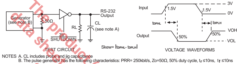
Figure 2. Driver Propagation and Skew
