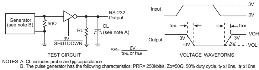
Figure 1. Driver Slew Rate
