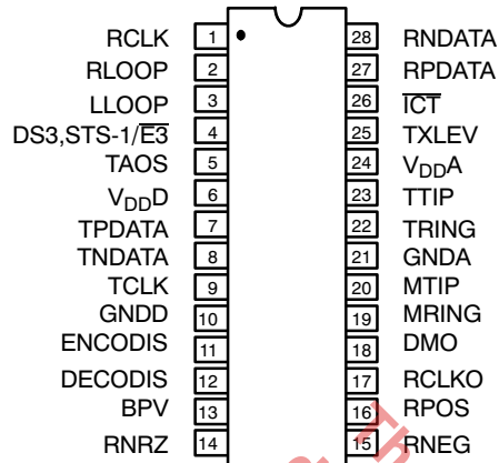
28 Lead PDIP (0.600")
