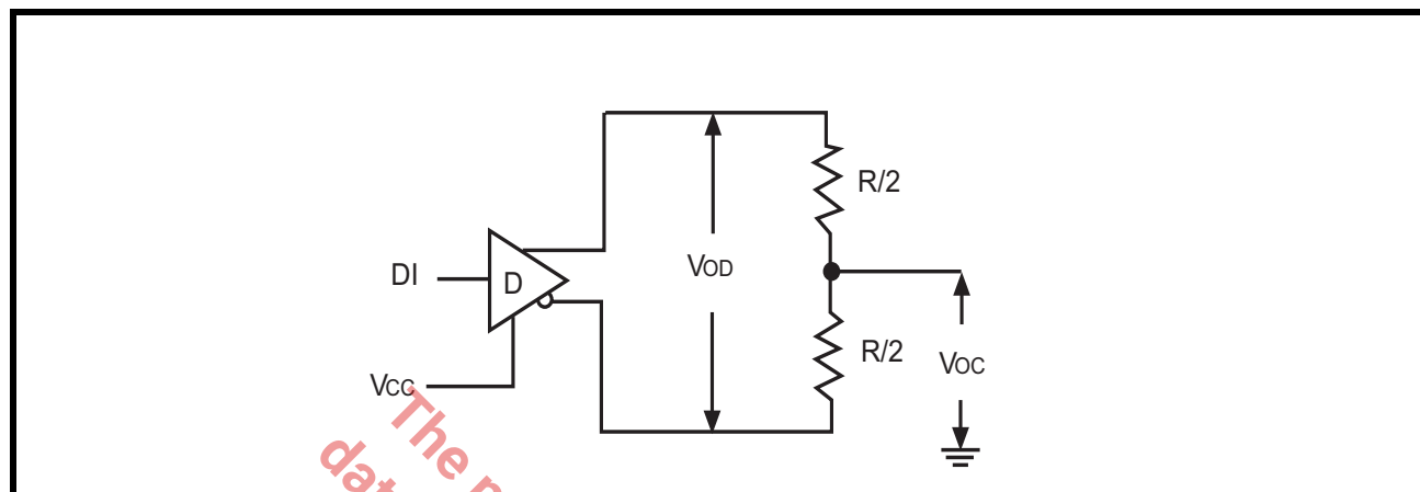
FIGURE 3. DRIVER DC TEST CIRCUIT
