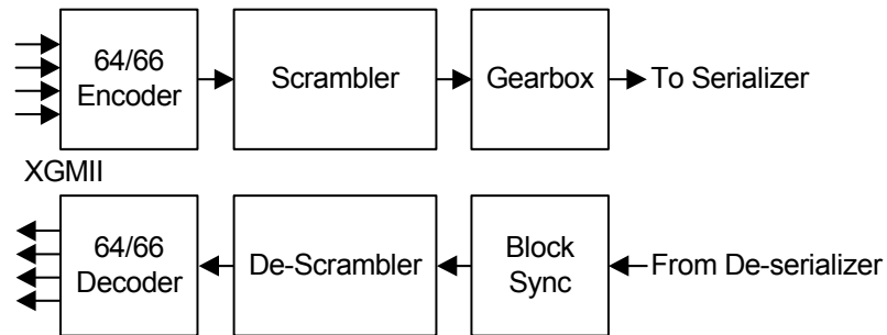
Figure 21: 10GBASE-R PCS
