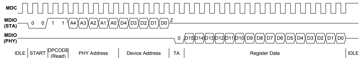
Figure 7: Typical MDC/MDIO Write Operation
