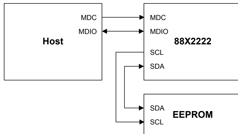
Figure 11: MDC/MDIO Bridging
