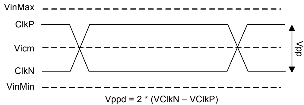
Figure 45: Reference Clock Input Waveform
