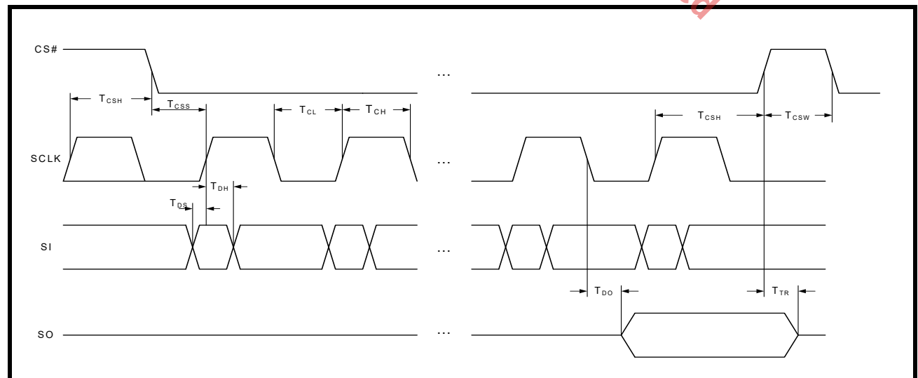
FIGURE 29. SPI-BUS TIMING
