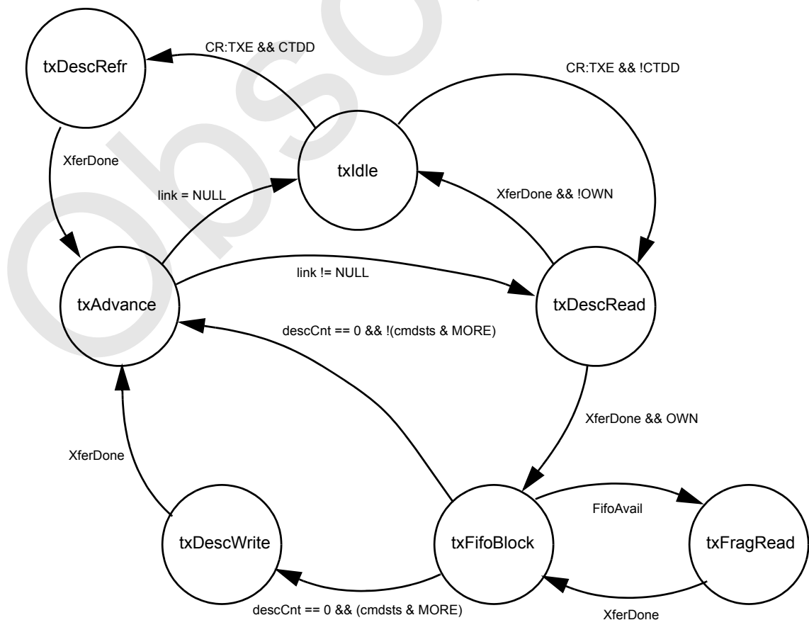
Figure 5-5 Transmit State Diagram
