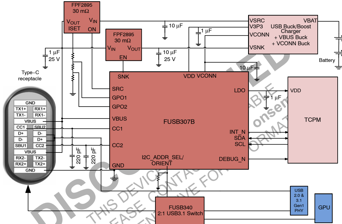
Figure 2. FUSB307B Typical Mobile Computing Application
