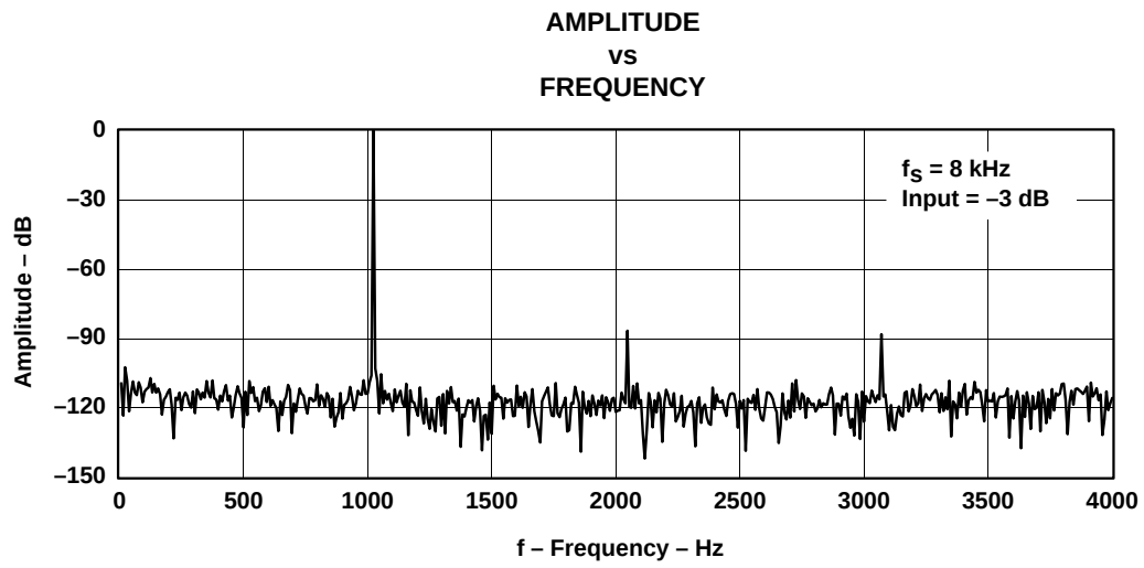
Figure 5-5. FFT-DAC Channel
