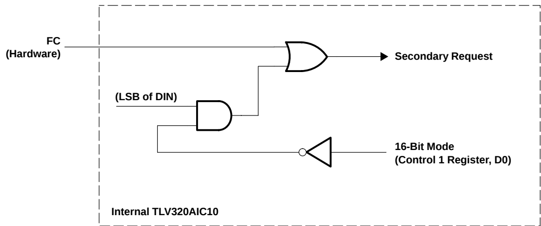
Figure 3–2. Hardware and Software Secondary Communication Request
