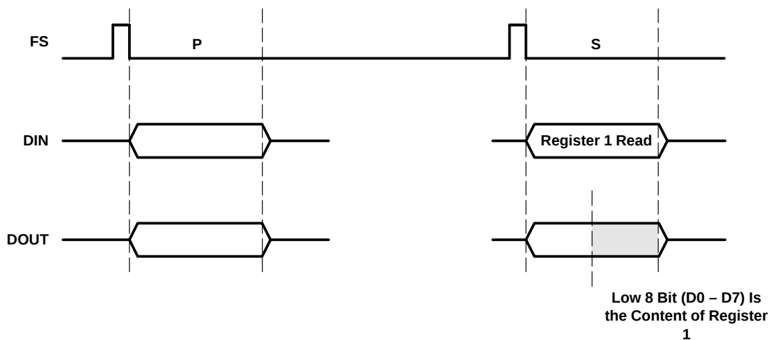
Figure 3–3. Device 3/Register 1 Read Operation Timing Diagram
