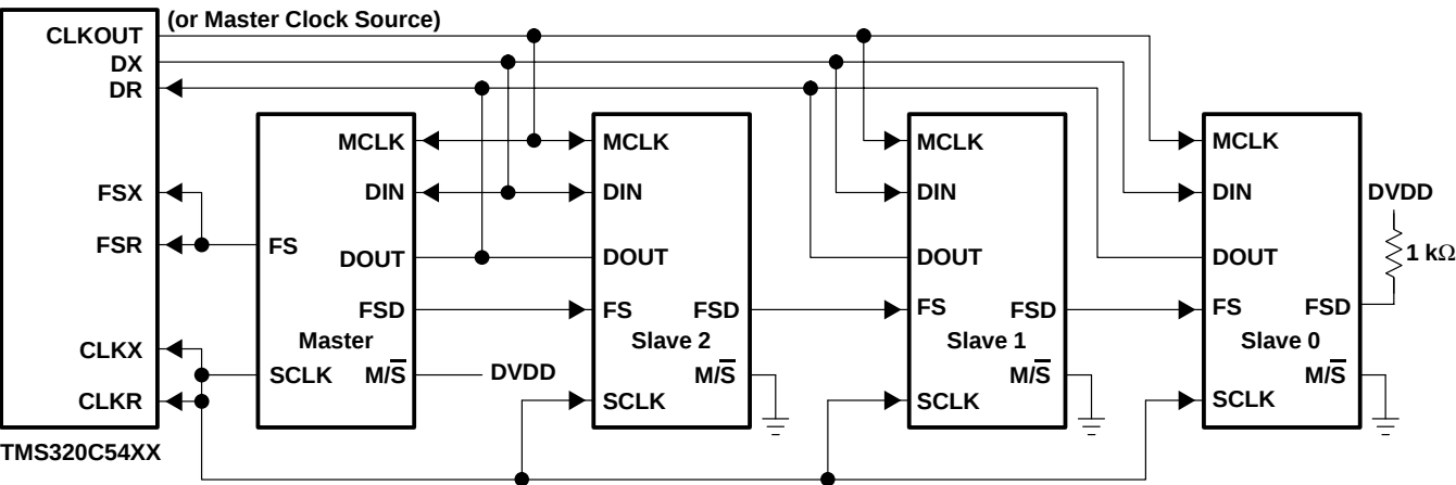
Figure 2–14. Cascade Mode Connection (to DSP Interface)
