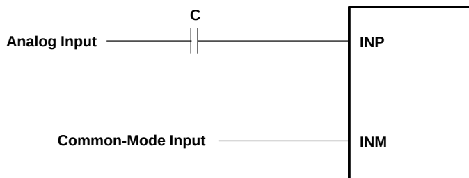
Figure 2–18. Single-Ended Input
