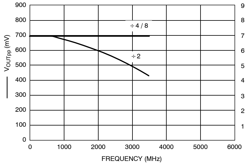
Figure 4. F_{max}
