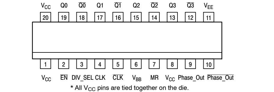
Figure 1. Pinout Assignment (Top View)
