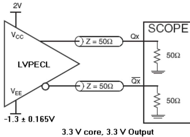
Figure 4. Typical Test Setup and Termination for Evaluation. The V_{CC} of 2.0 \text{ V} and V_{EE} of -1.3 \pm 0.165 \text{ V} Split supply allows a direct connection to an oscilloscope 50 \Omega impedance input module. Also reference AND8020.
