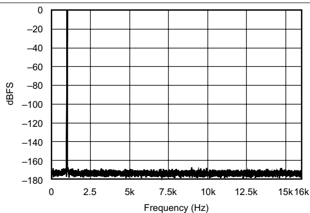
Figure 23. FFT With 1-kHz Input Tone at 0 dBFS
