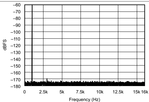
Figure 24. FFT With 1-kHz Input Tone at -60 dBFS
