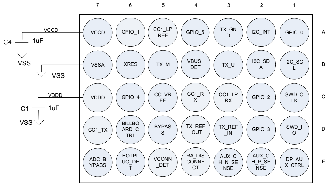
Figure 5. 35-ball WLCSP Example
