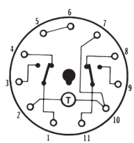
OFF DELAY
