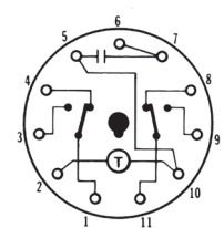
INTERVAL/ON-DELAY
