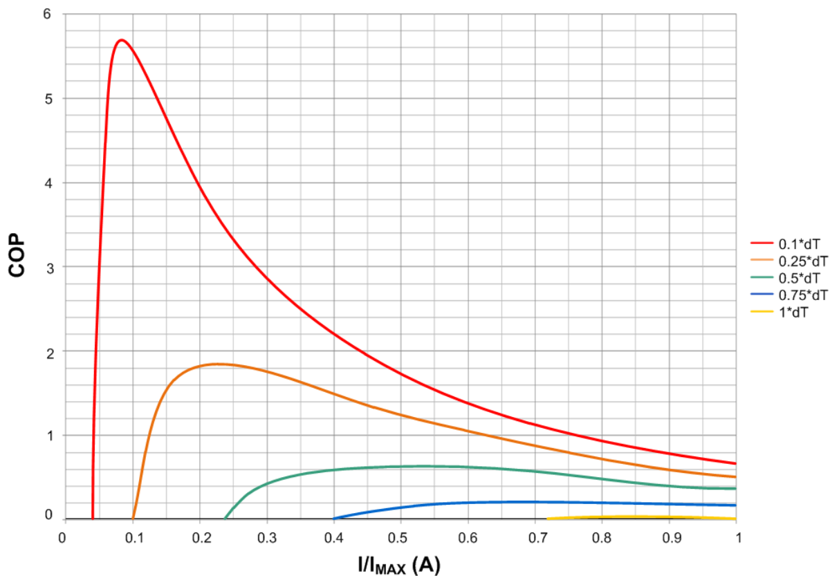
Figure 17. COP vs. I/I_{MAX}
