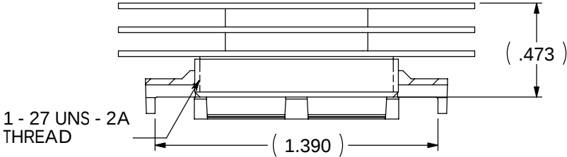
SECTION B-B
