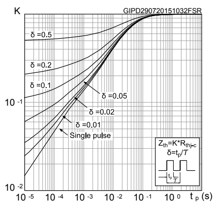
Figure 15. Thermal impedance
