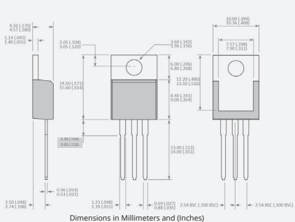
TO-220 3-Lead
