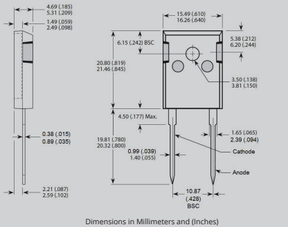
TO-247 2-Lead
