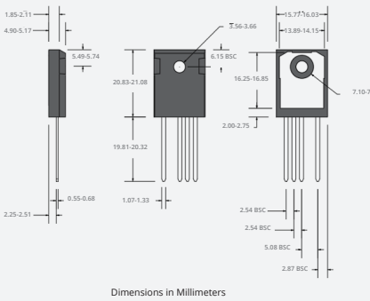
TO-247 4-Lead
