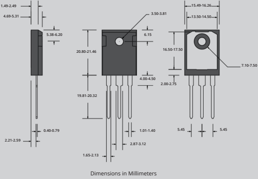
TO-247 3-Lead
