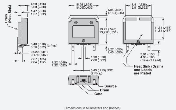
TO-268 (D3PAK)
