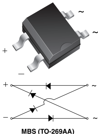
MBS (TO-269AA)
