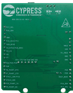
Figure 2: CYBT-423028-EVAL Bottom View
