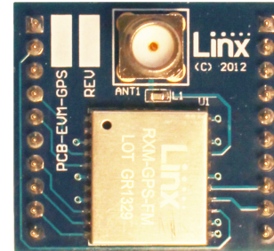
Figure 1: FM Series Evaluation Module
