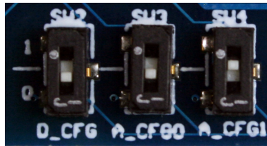
Figure 5: The Evaluation Board Input Interpretation Selection Switches
