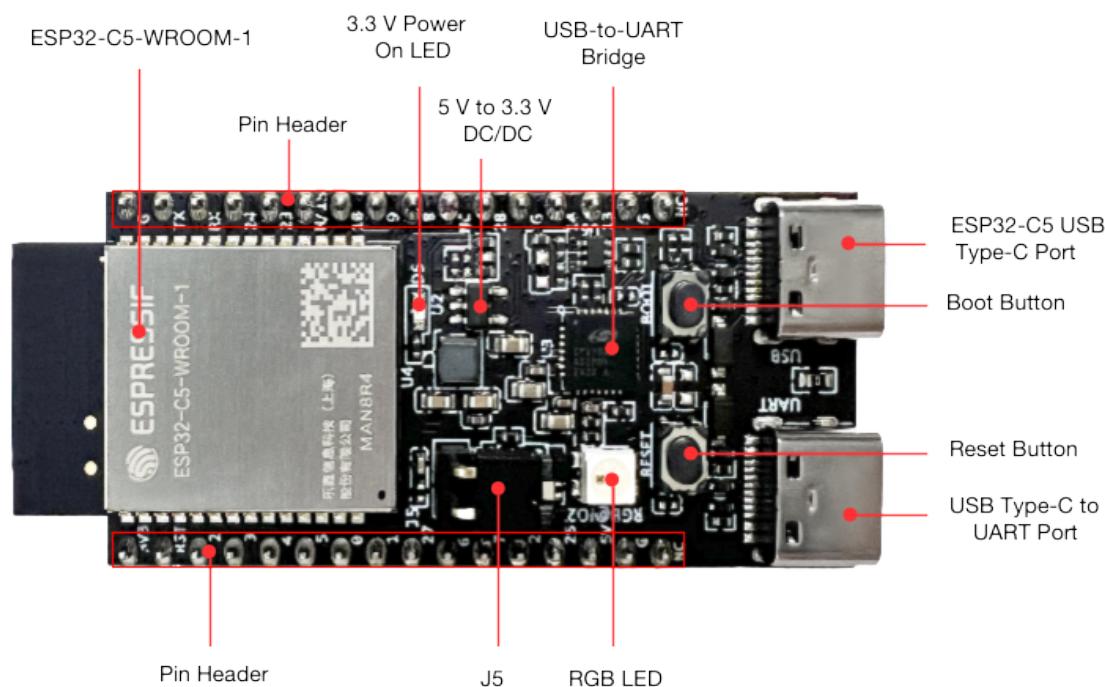
Fig. 6: ESP32-C5-DevKitC-1 - front
