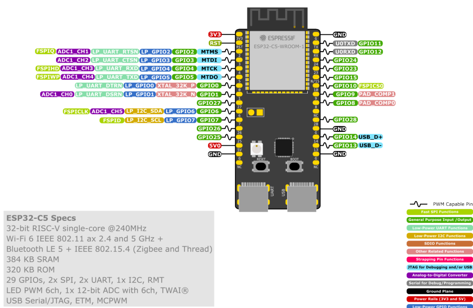
Fig. 8: ESP32-C5-DevKitC-1 Pin Layout (click to enlarge)
