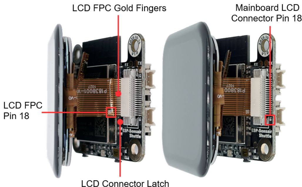
Fig. 8: LCD Screen Cable Installation Diagram (Click to enlarge)
