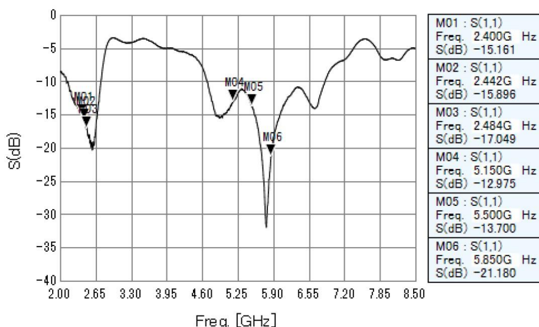
Figure 9 – Return Loss for Certified Trace Antenna
