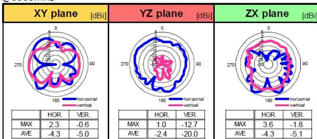
Figure 12 – Directivity for Certified Trace Antenna
