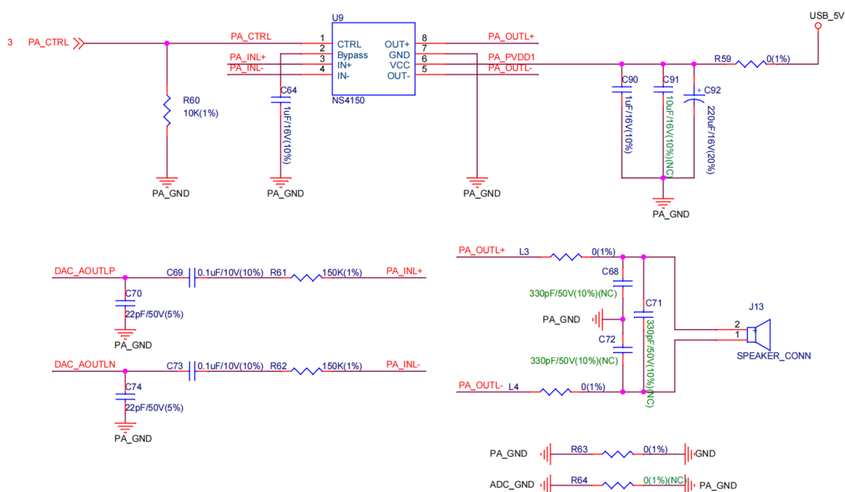
Fig. 17: SP32-S3-LCD-Ev-Board - AEC PA Output (Click to Enlarge)
