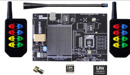
Figure 1: MS Long-Range Handheld Transmitter Master Development System
