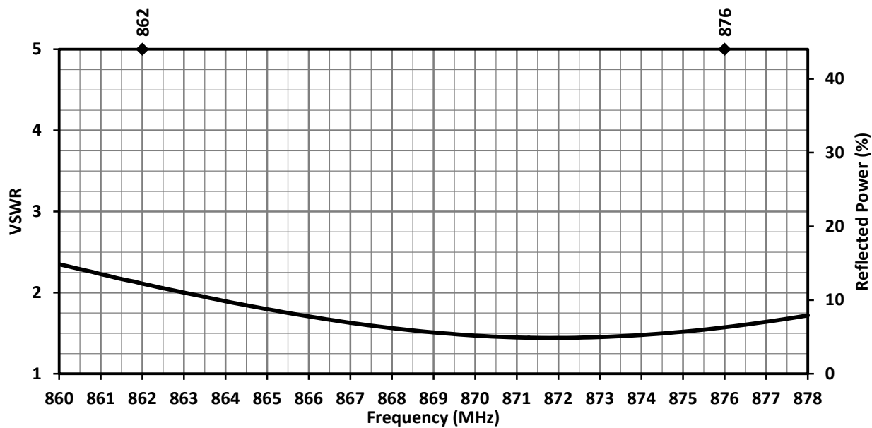
Figure 1. ANT-868-uSP410 VSWR
