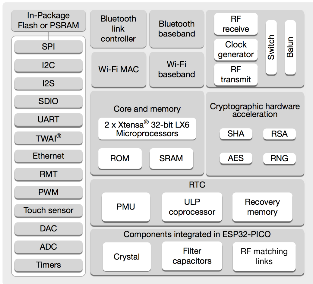
Figure 1: ESP32-PICO Functional Block Diagram
