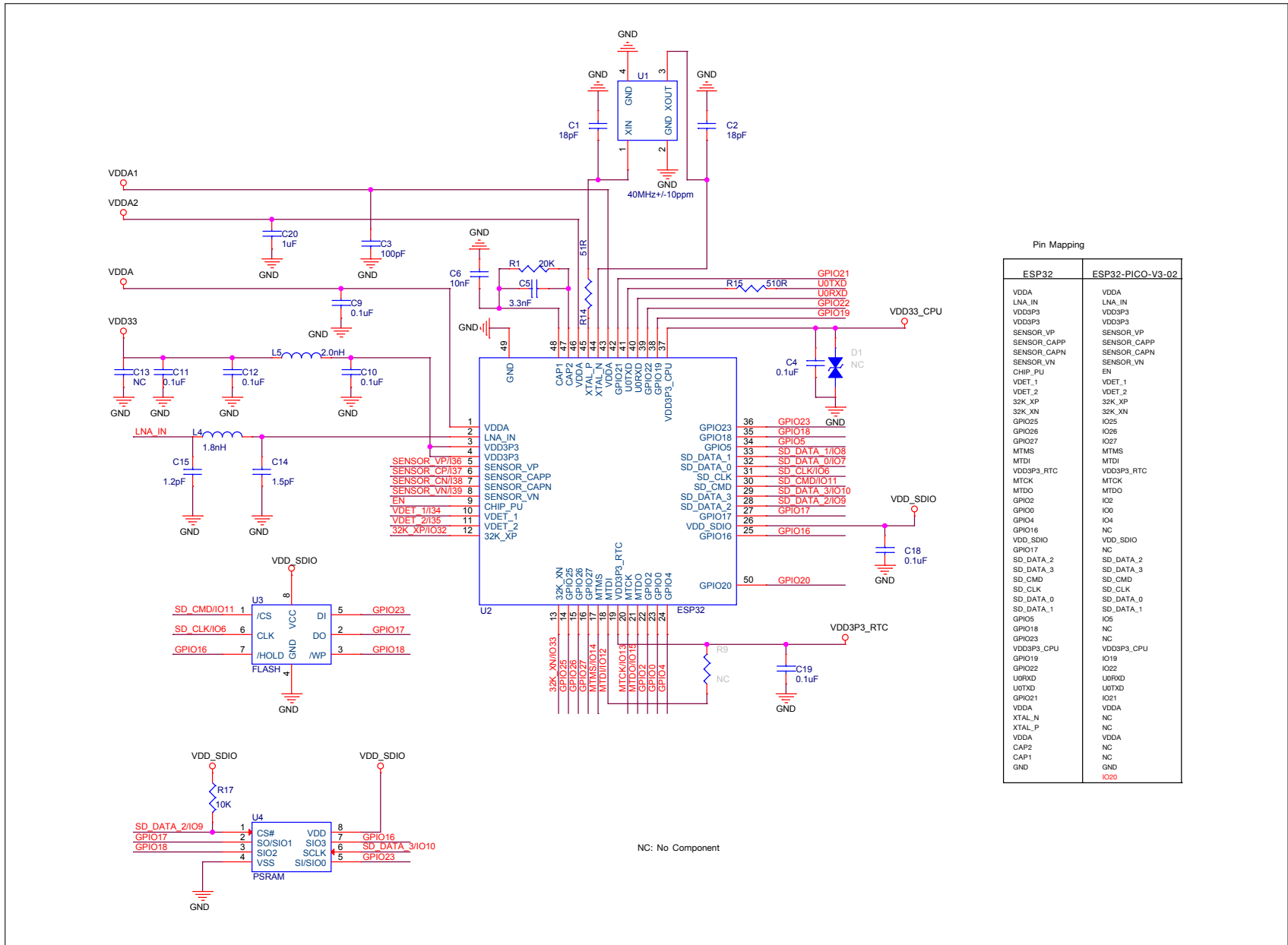
Figure 9: ESP32-PICO-V3-02 Schematics
