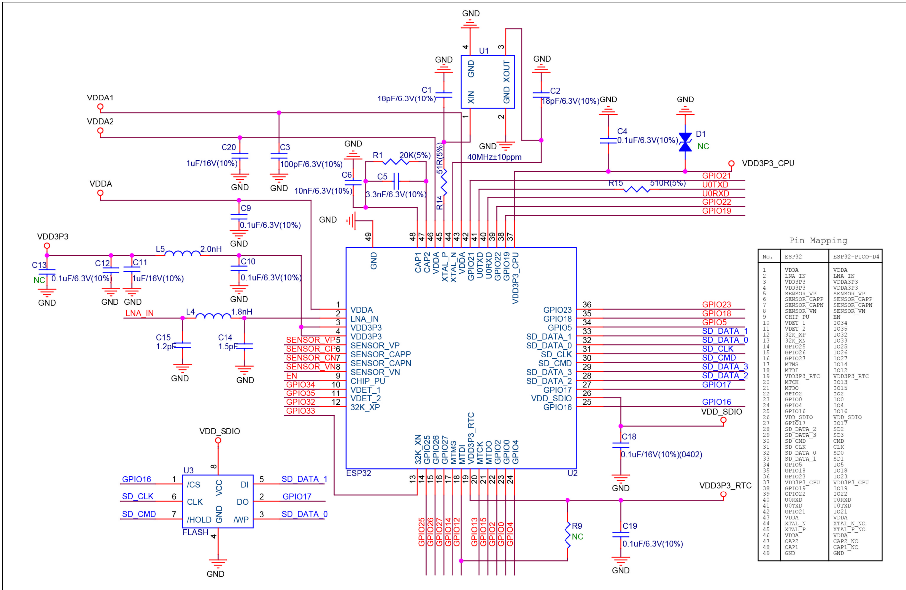
Figure 7: ESP32-PICO-D4 Schematics
