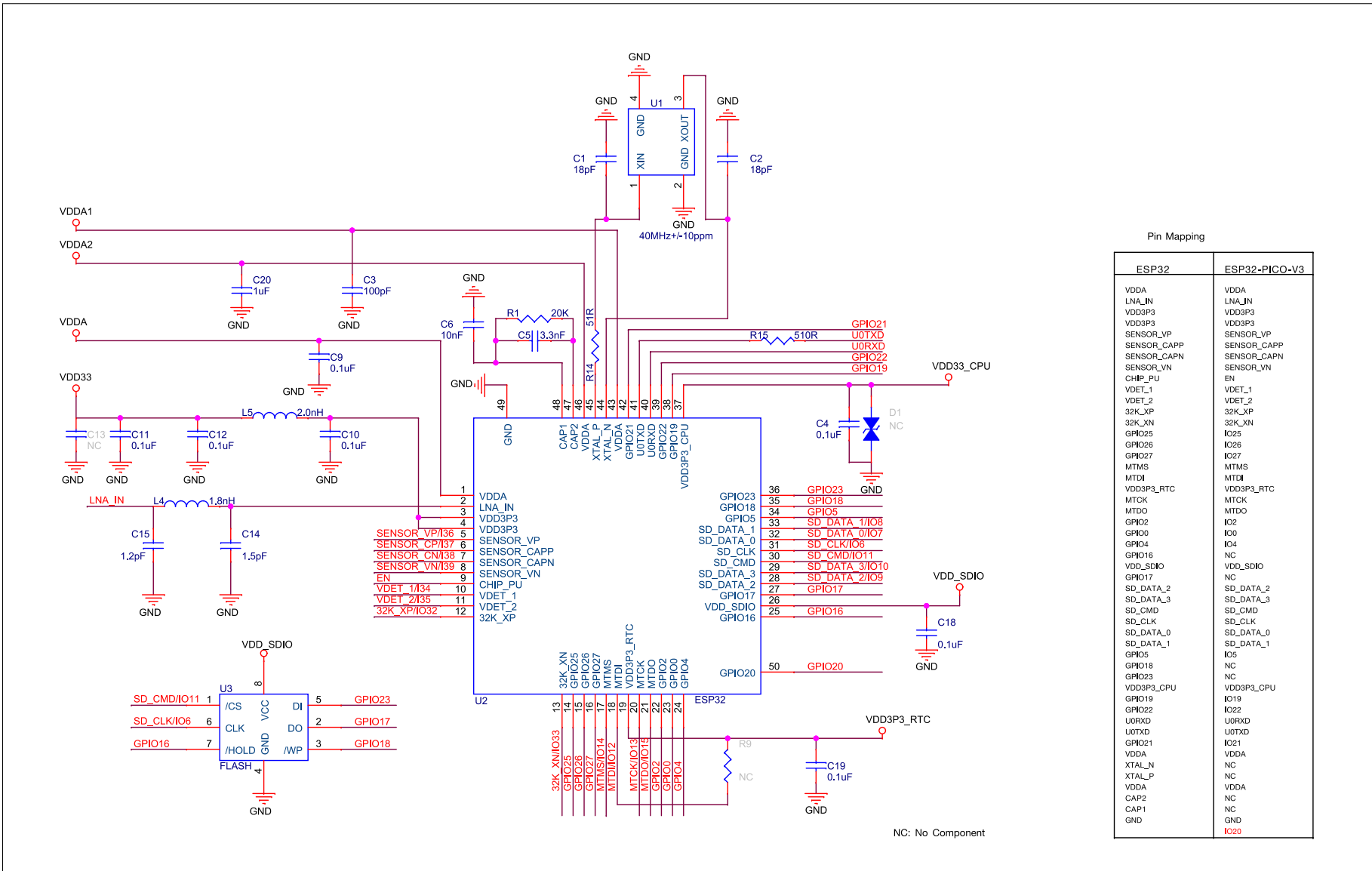
Figure 8: ESP32-PICO-V3 Schematics
