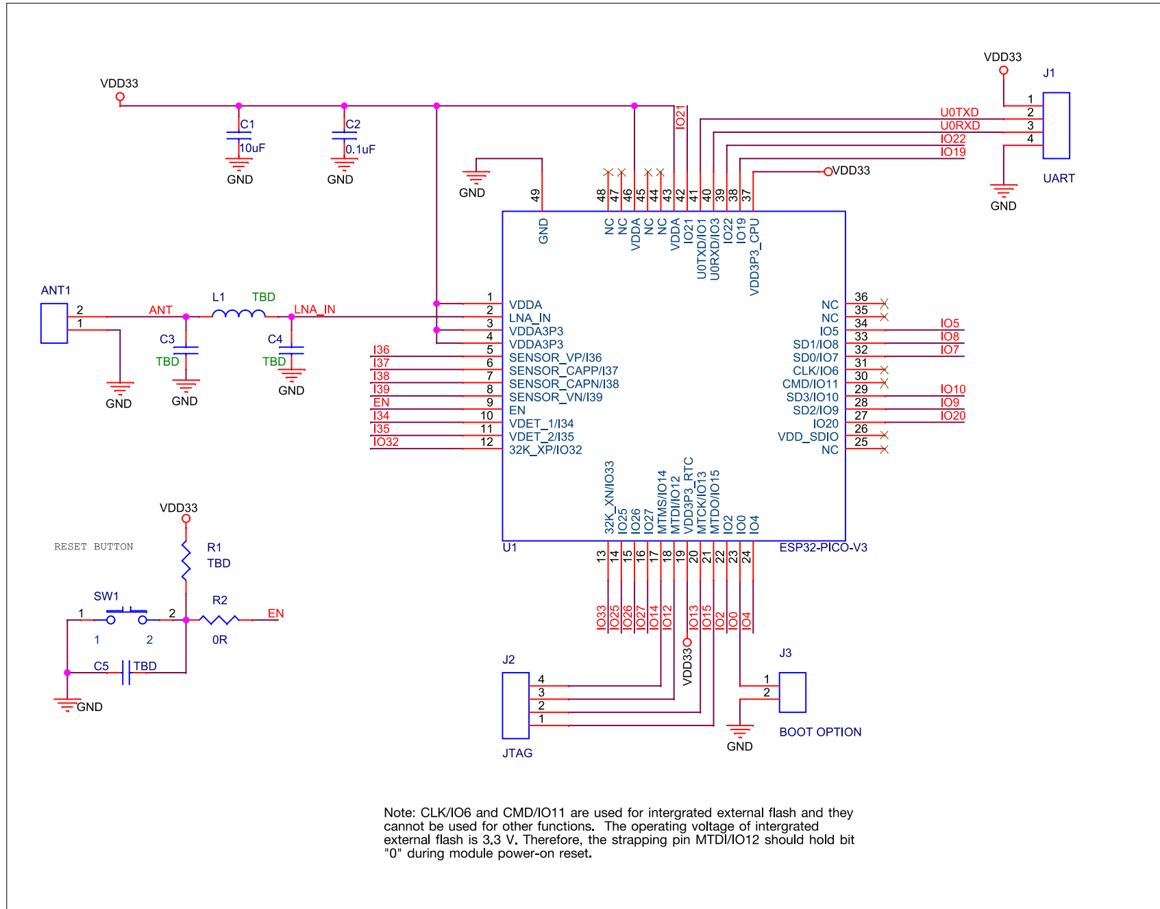
Figure 11: ESP32-PICO-V3 Peripheral Schematics
