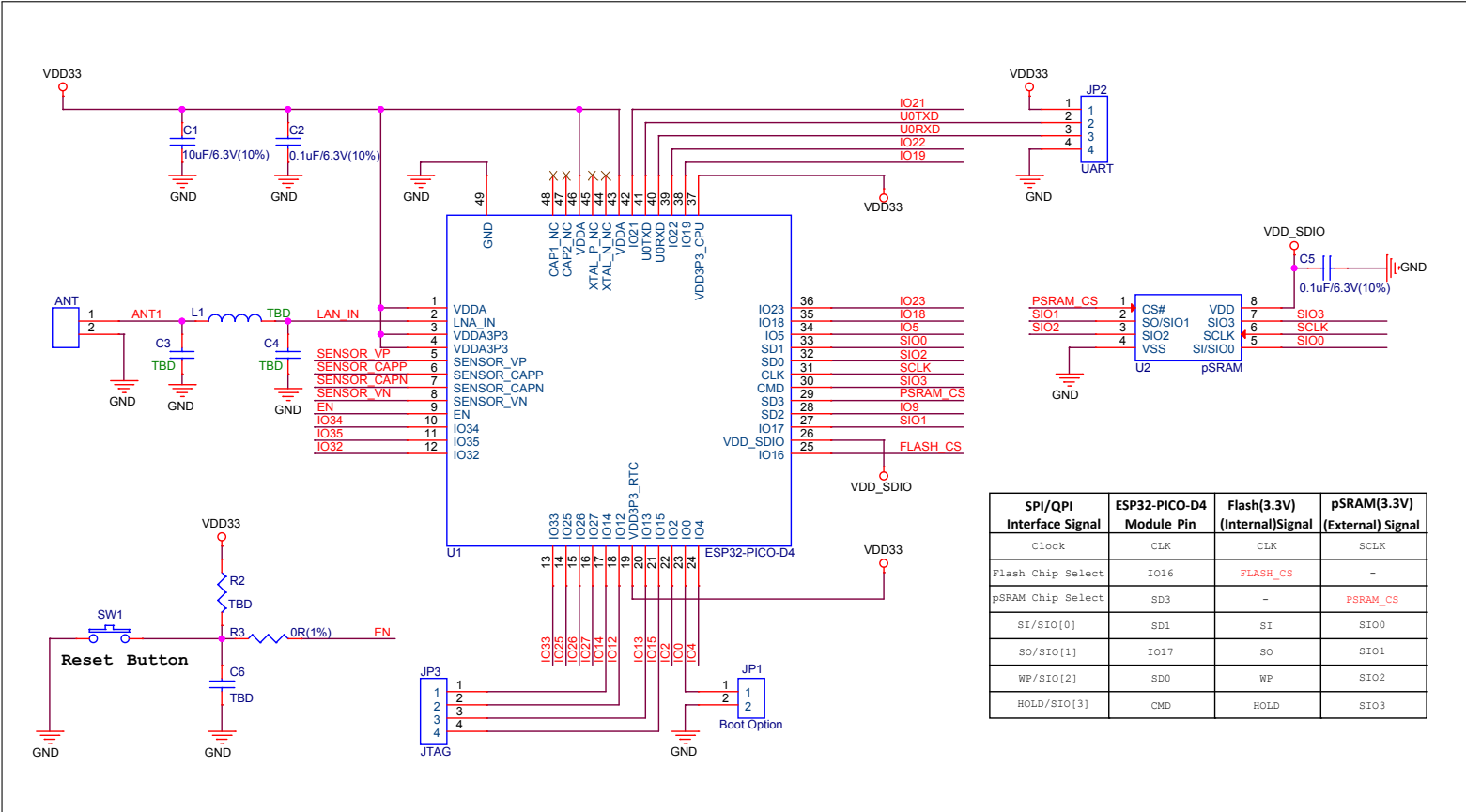
Figure 10: ESP32-PICO-D4 Peripheral Schematics
